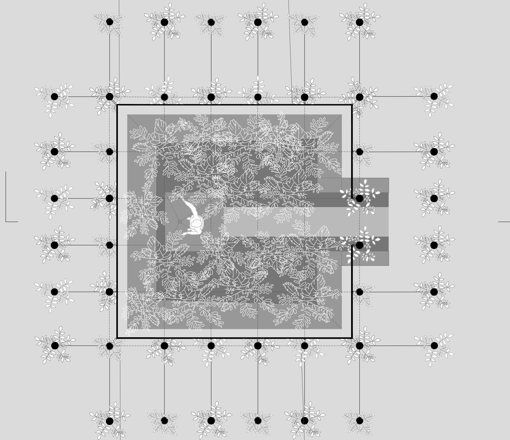
Planta ducha invernadero / Greenhouse shower floor plan
