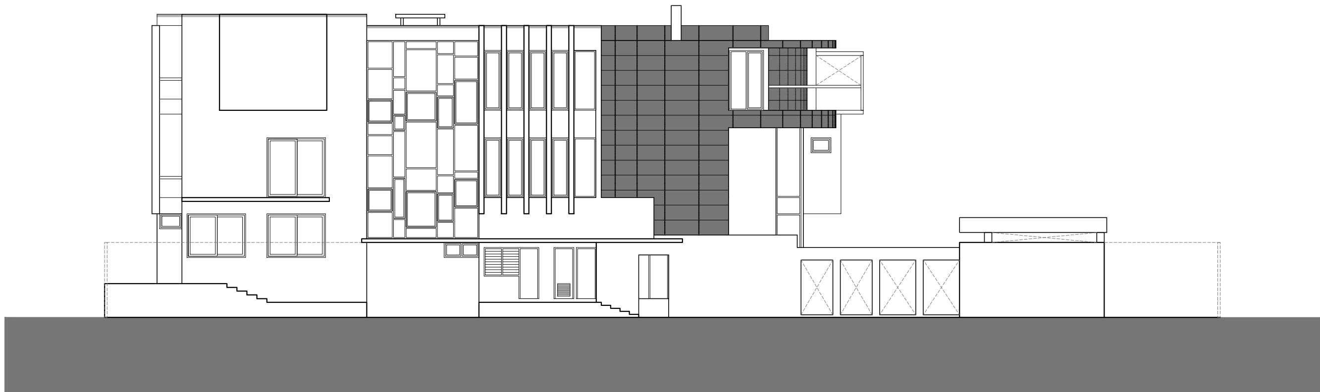
NORTH ELEVATION
