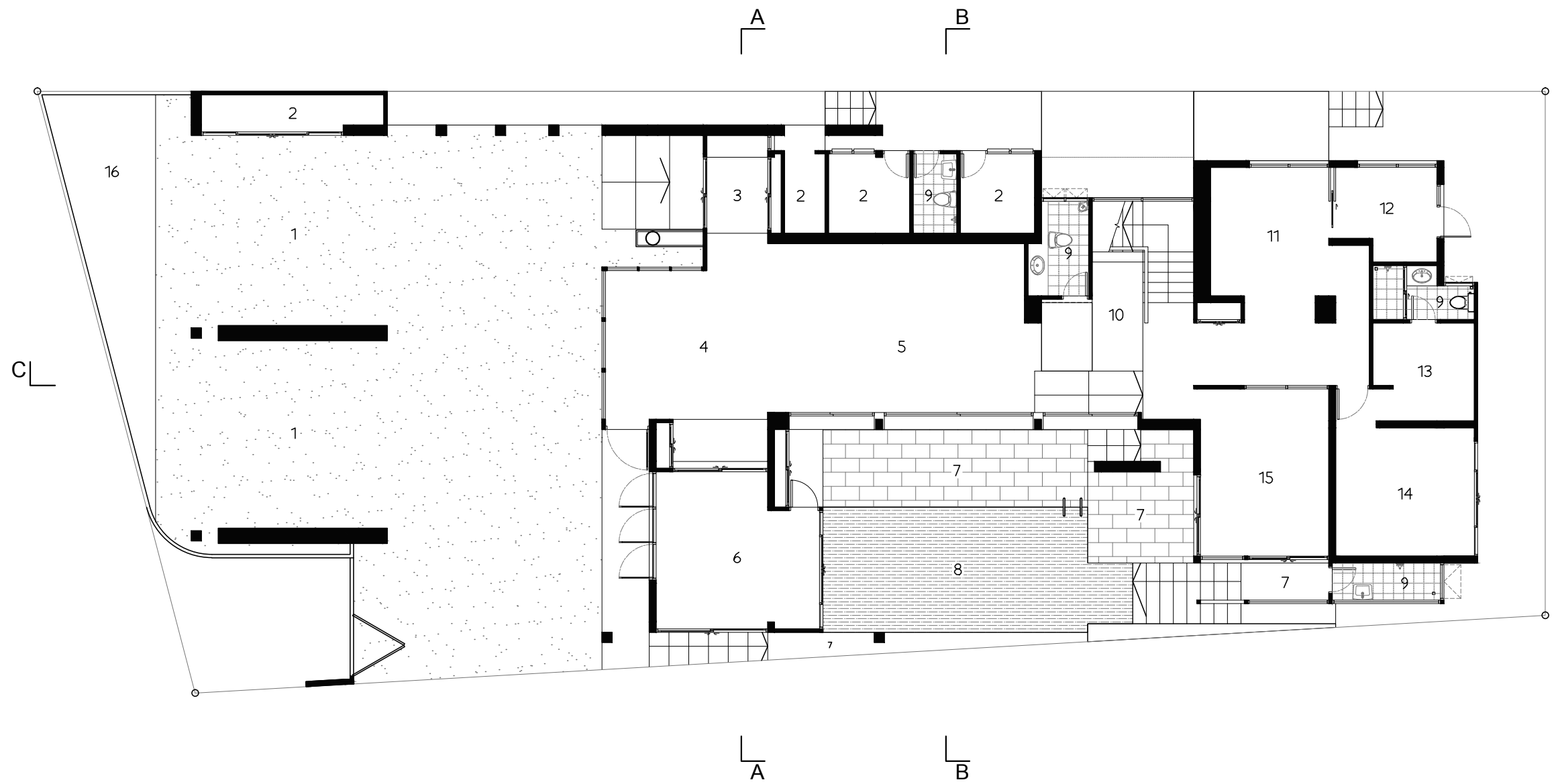
N FIRST FLOOR PLAN
