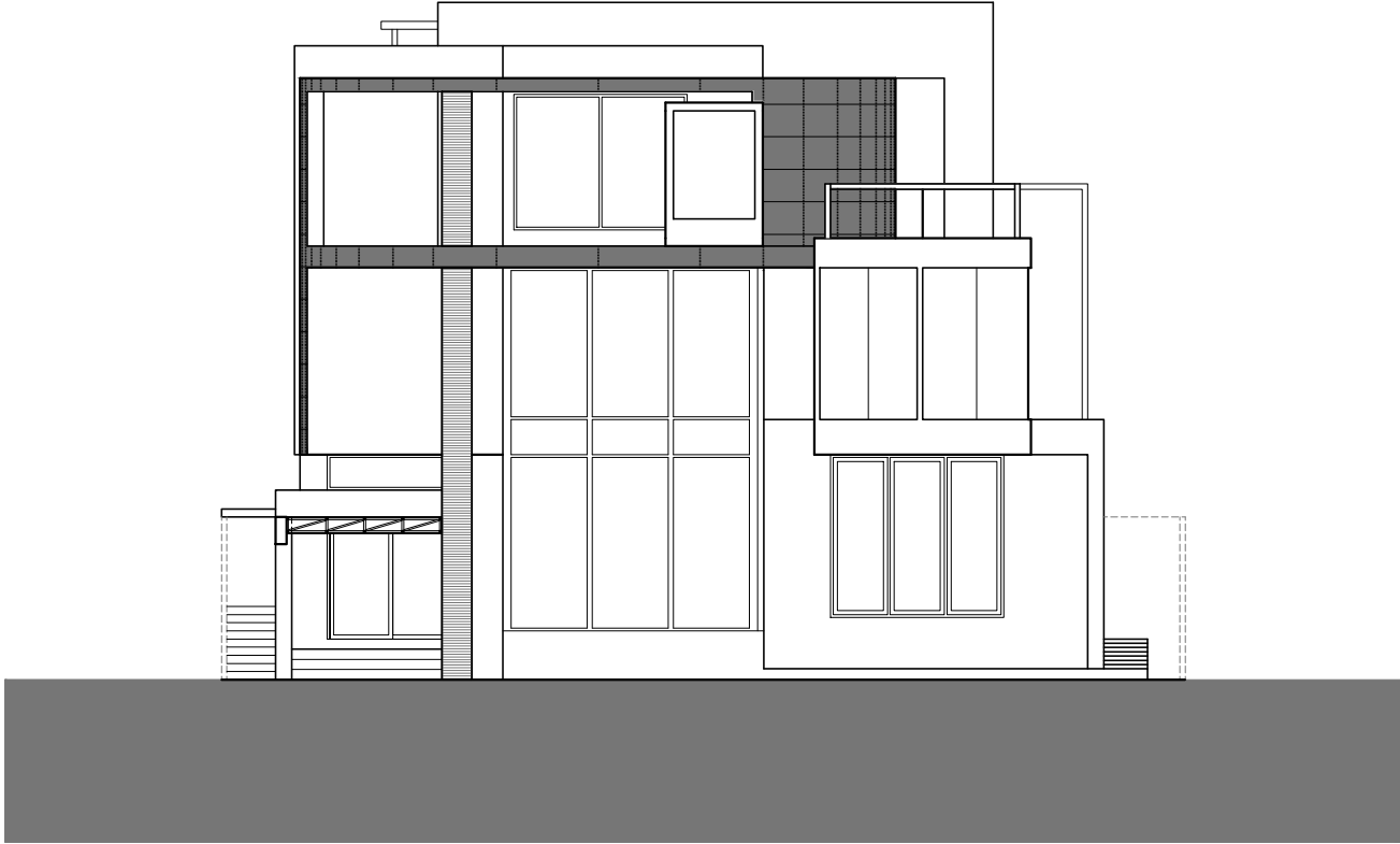
WEST ELEVATION
