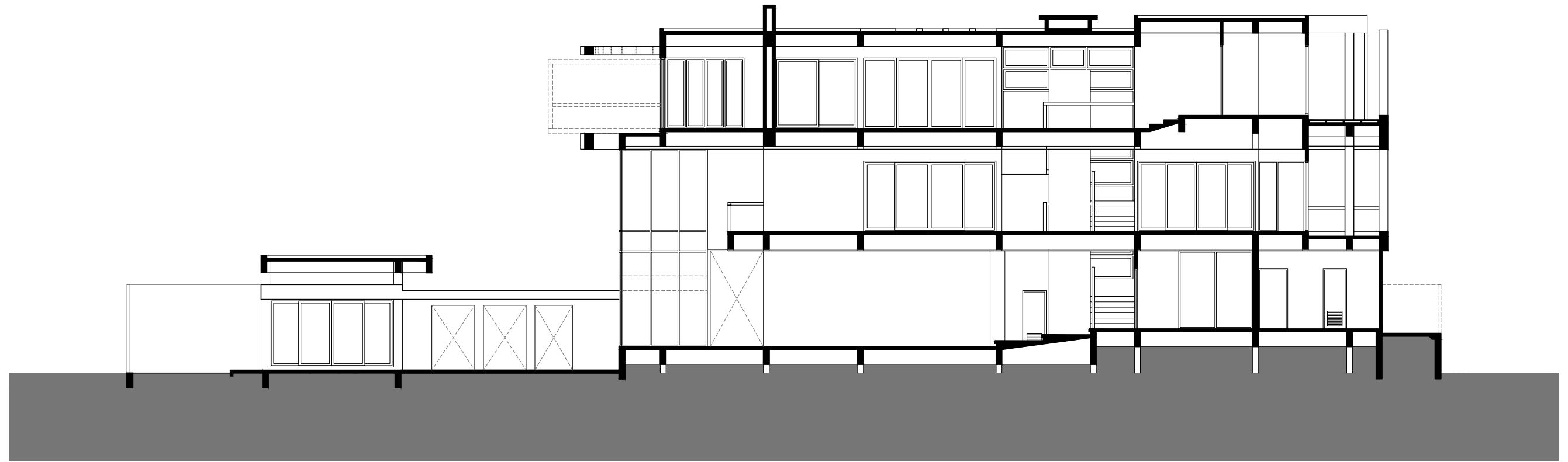
C-C SECTION
