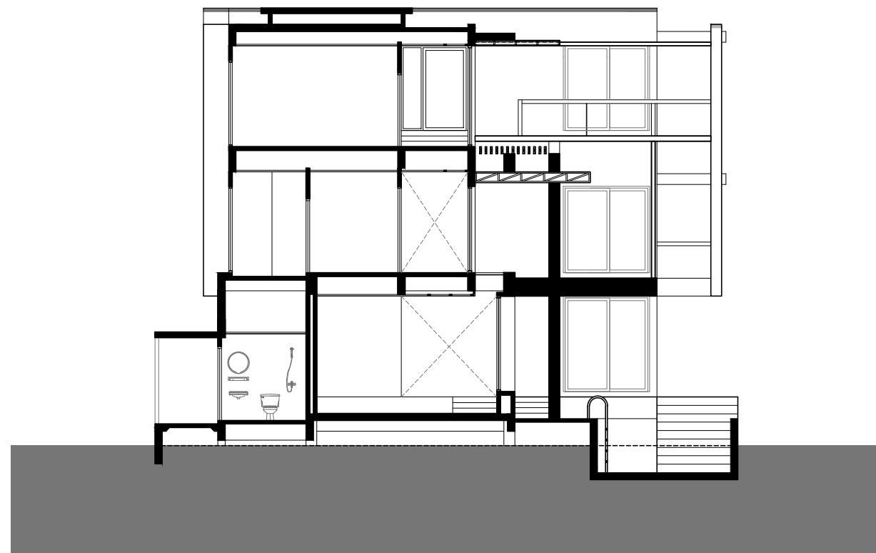
B-B SECTION
