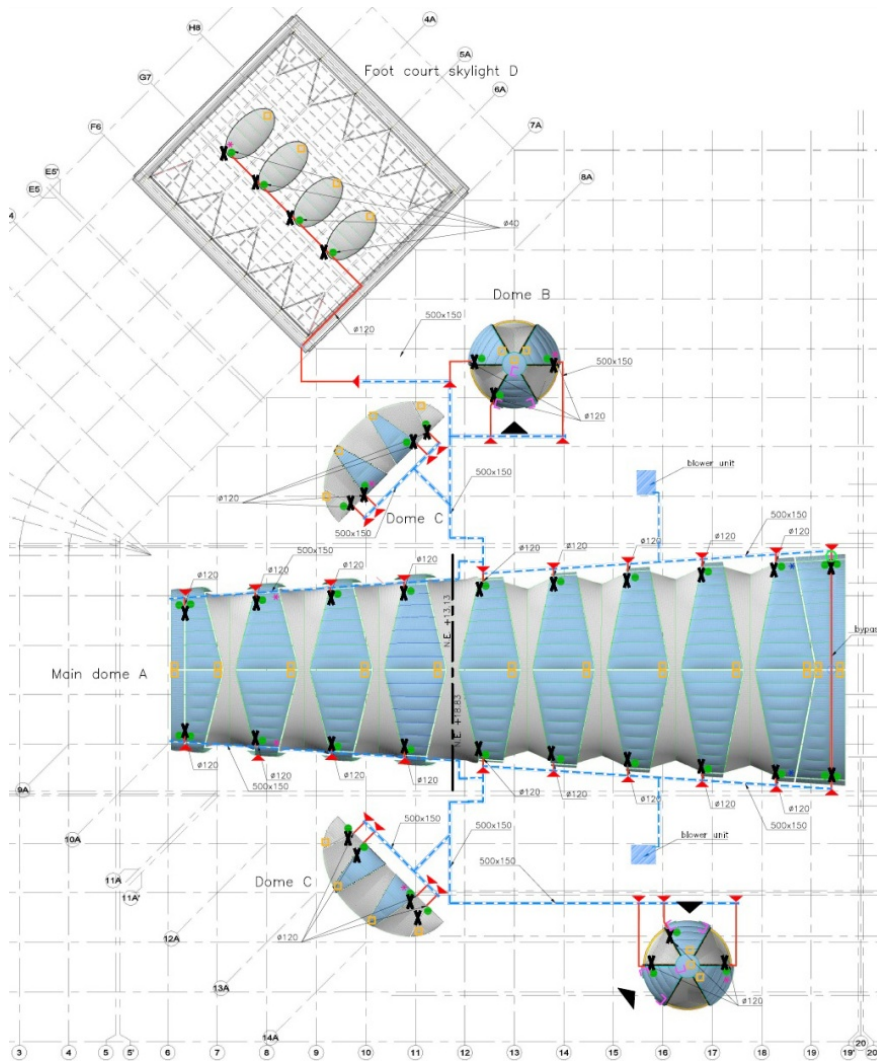
Layout plan of shopping center including air supply Drawing: 05_luftversorgung.jpg
