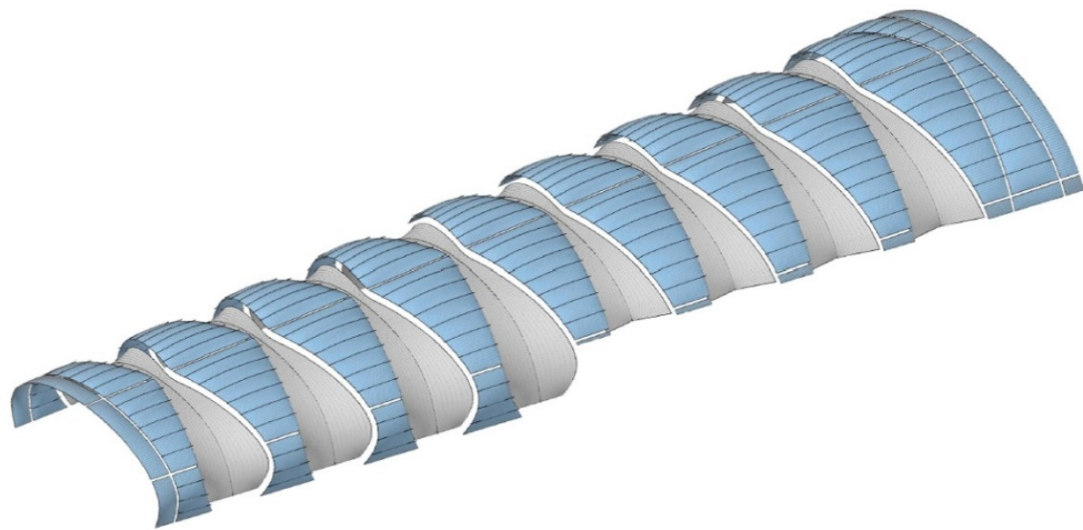
Attractive structure comprising rows of ETFE cushions and mechanically tensioned membrane – the main roof of the Titan Plaza Drawing: 01_maindome.jpg
