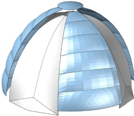
Roof with a circular layout Drawing + photo: 02_spericaldome.jpg; TITAN-DomoAscensor.JPG
