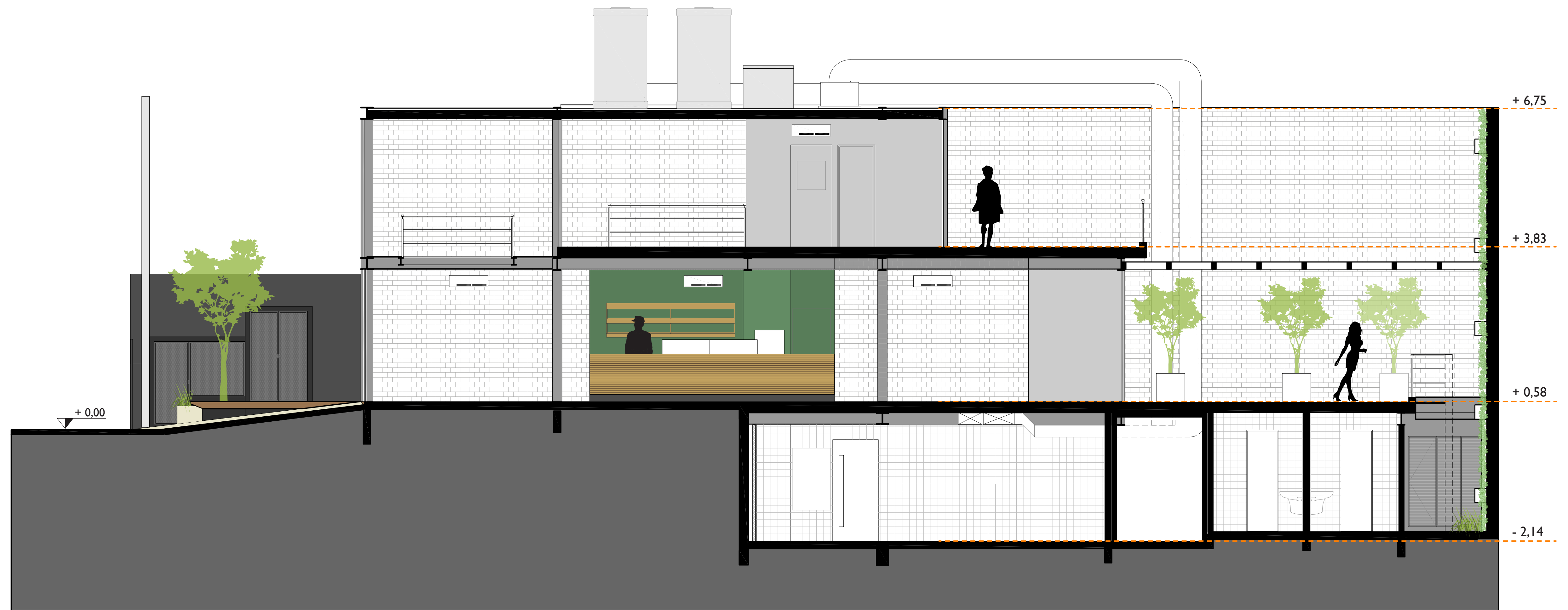
SECTION AA
