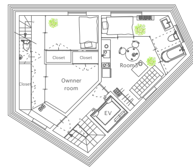
Sixth floor plan S=1:200
