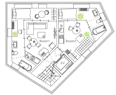
Third - Fifth floor plan S=1:200
