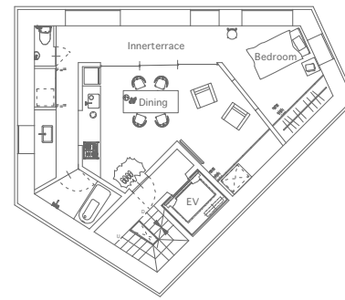
Second floor plan S=1:200
