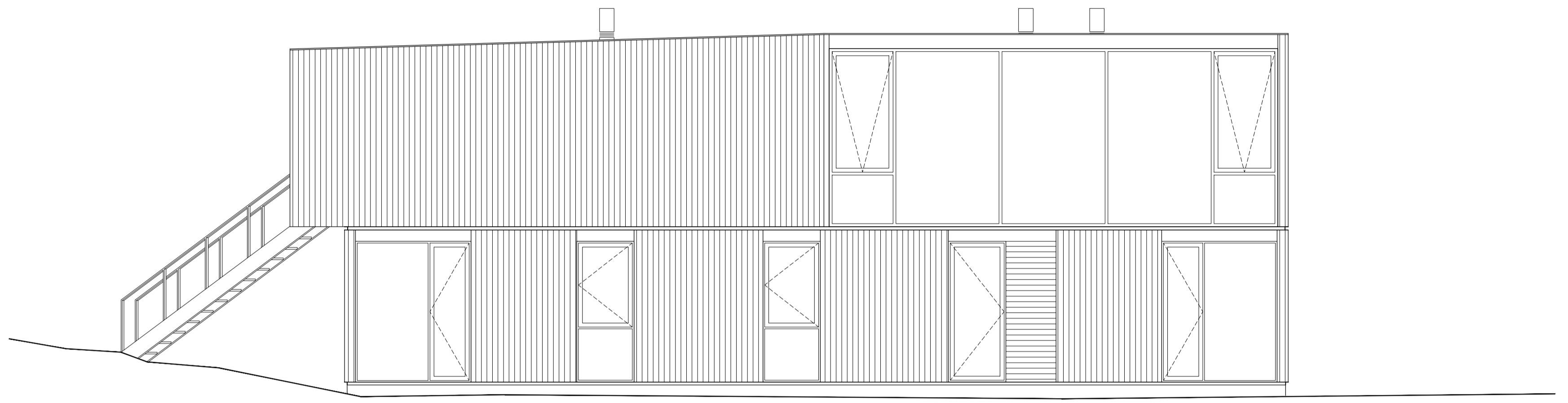
North Elevation
