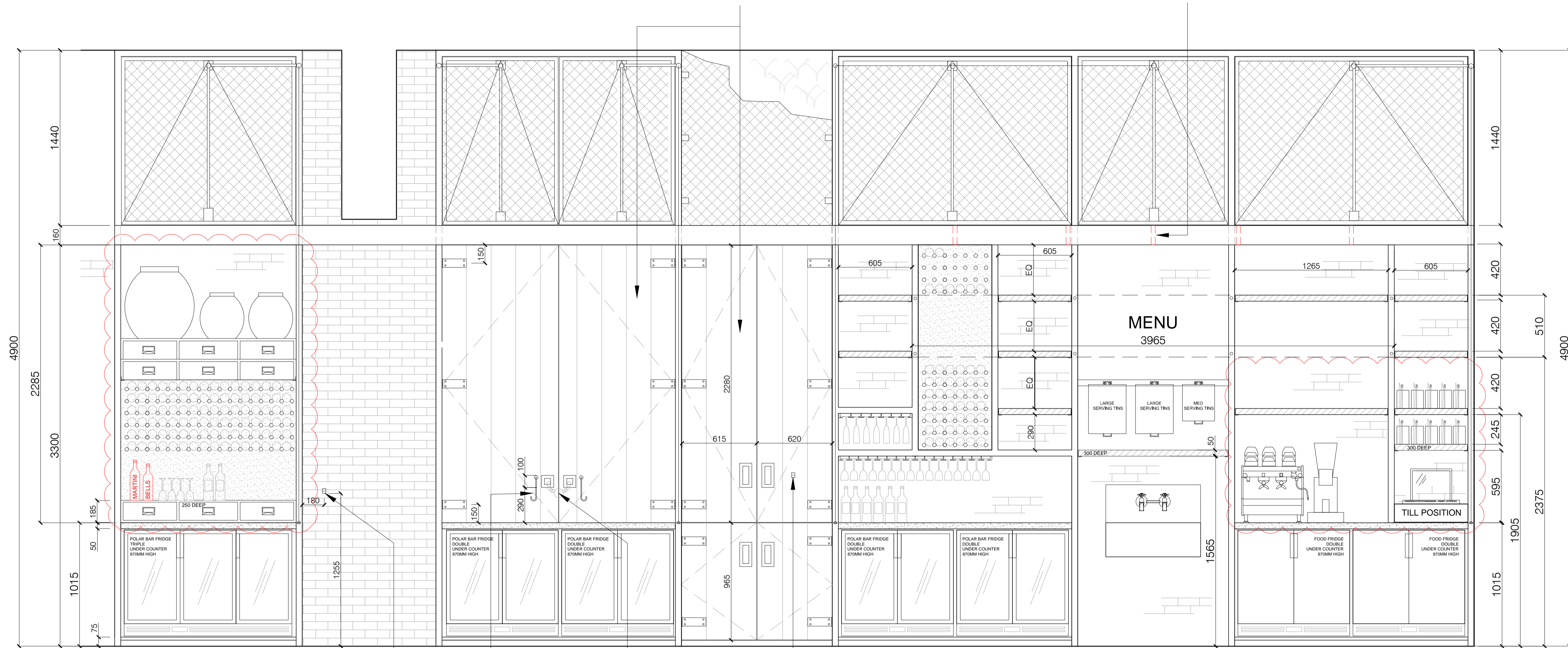
01 ELEVATION AA- BAR DOORS CLOSED 1:20 @ A1
