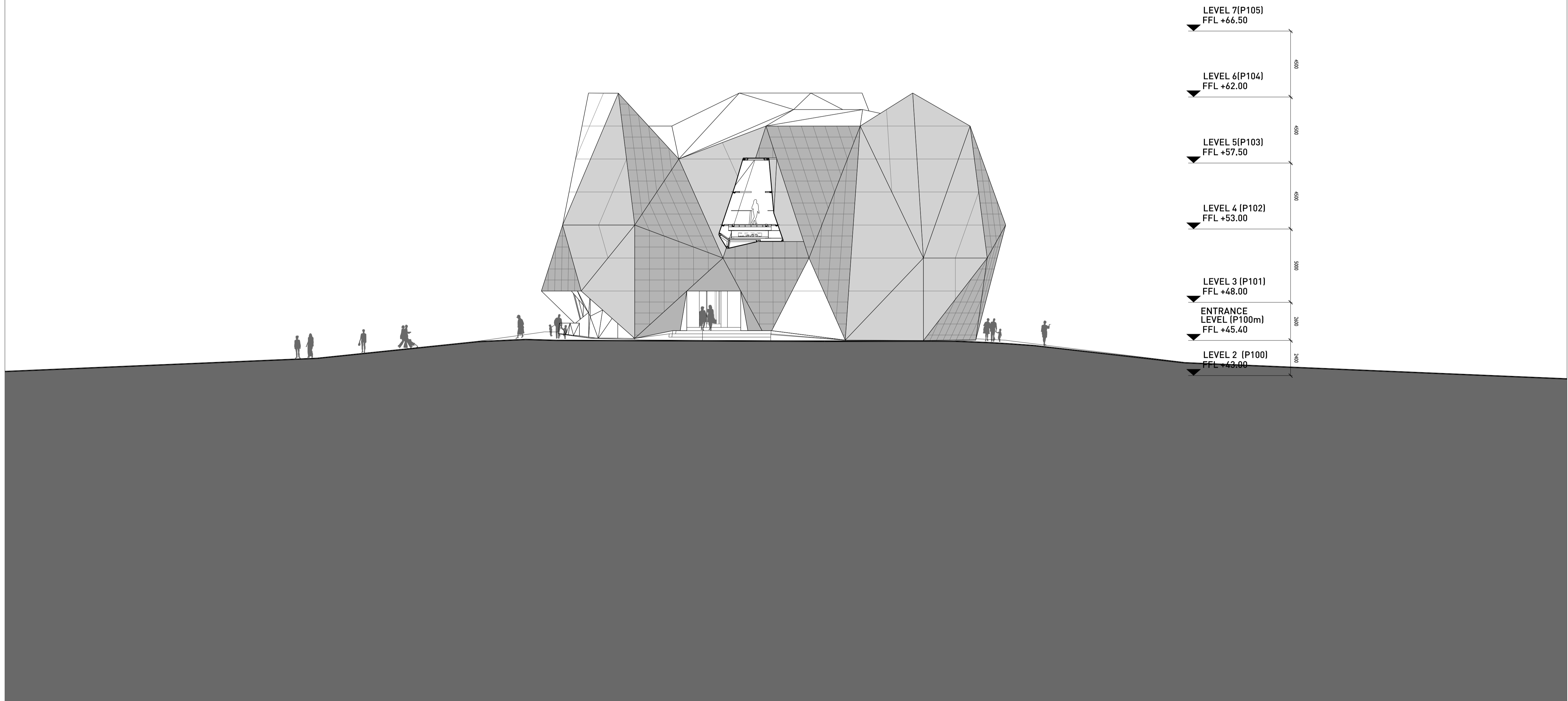
1 ELEVATION FROM GALLERY MAIN ENTRANCE GA/e304 SCALE 1:150
