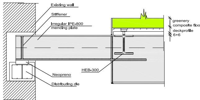
D1 DETAIL OF FRAME MEETING ENCLOSING WALL E:1/25
