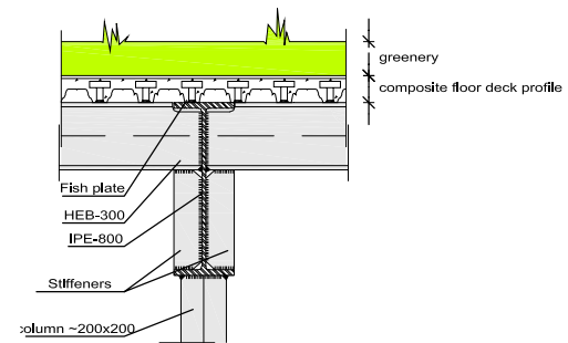
D3 DETAIL OF CENTRAL FRAME E:1/25
