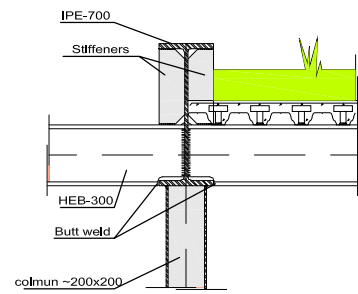
D2 DETAIL OF FACADE FRAME E:1/25
