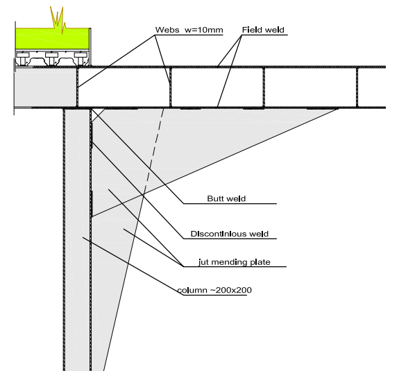
D4 DETAIL OF COLUMN IN COURTYARD E:1/25
