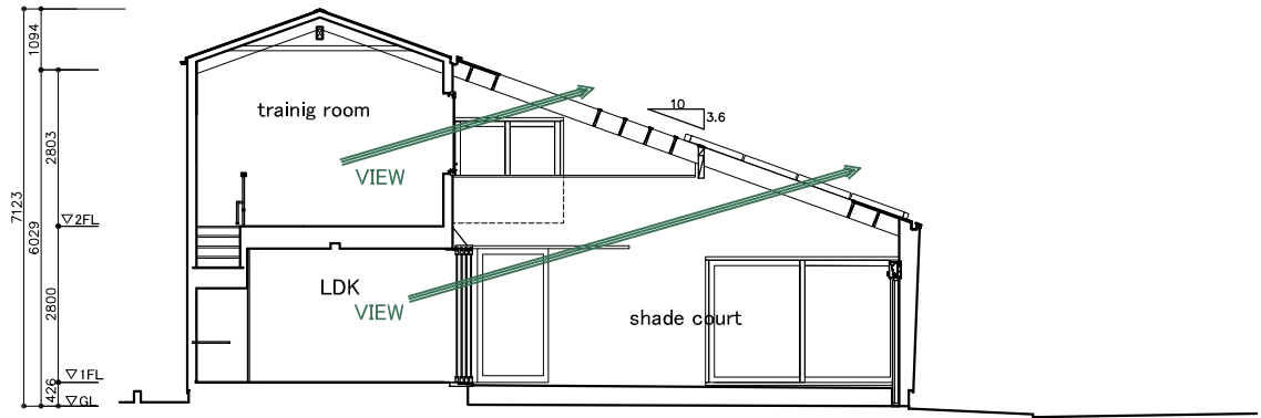
section S=1/150
