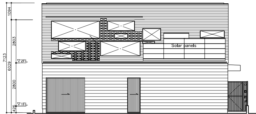
south elevation S=1/150
