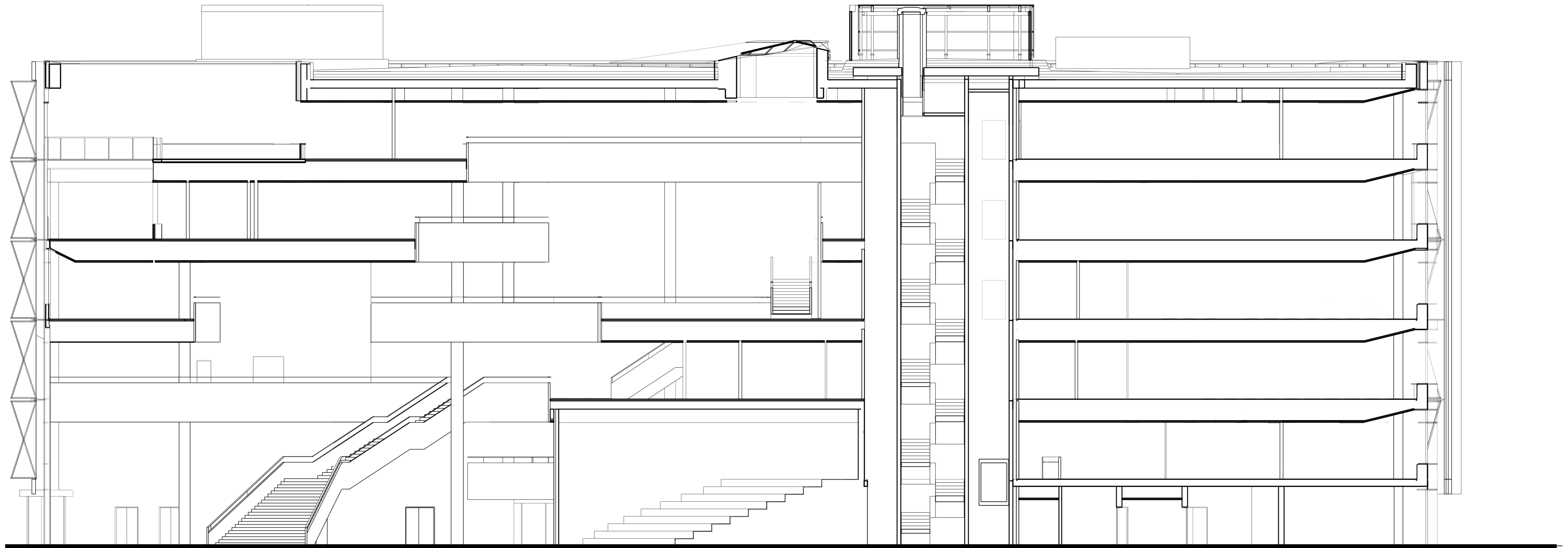
Section 1:100
