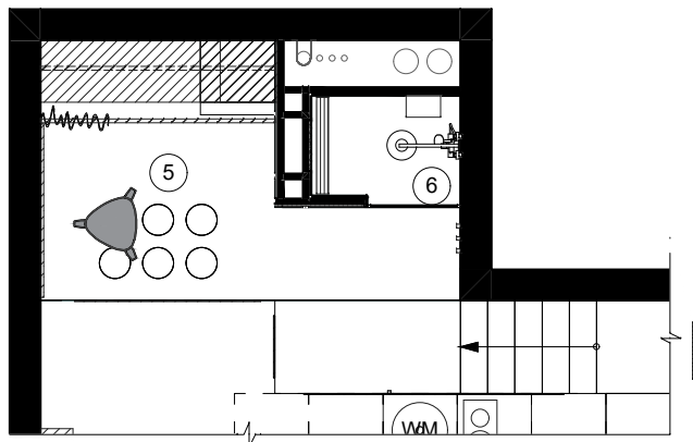
2d floor. +2,100 (1:50)
