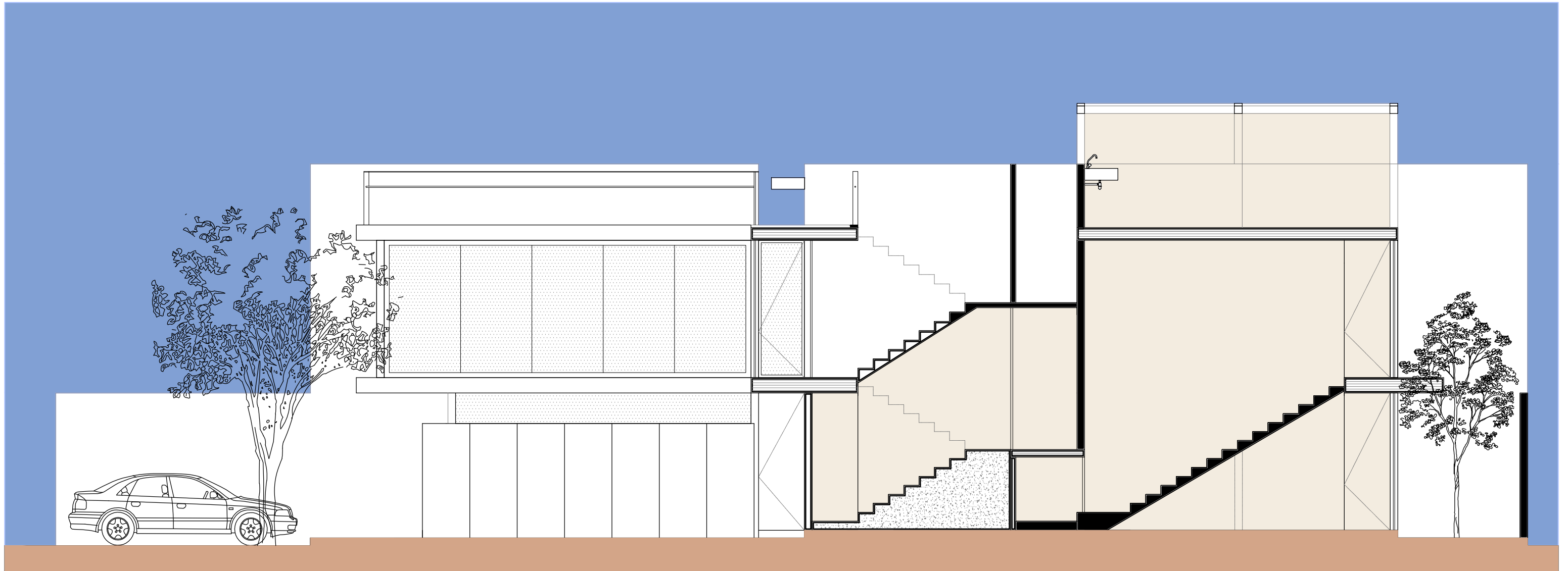
SECTION B-B'
