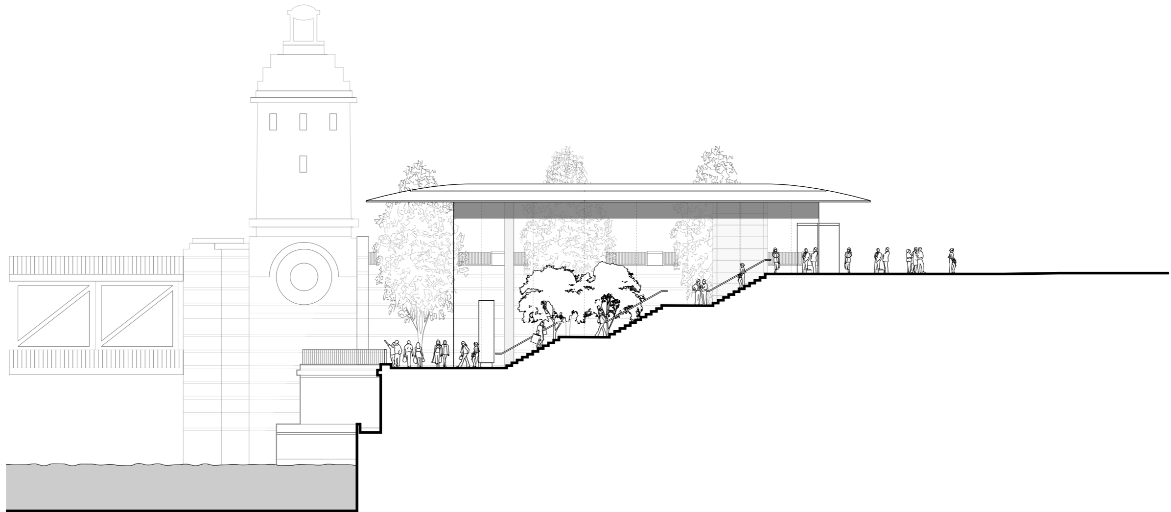
East Elevation
