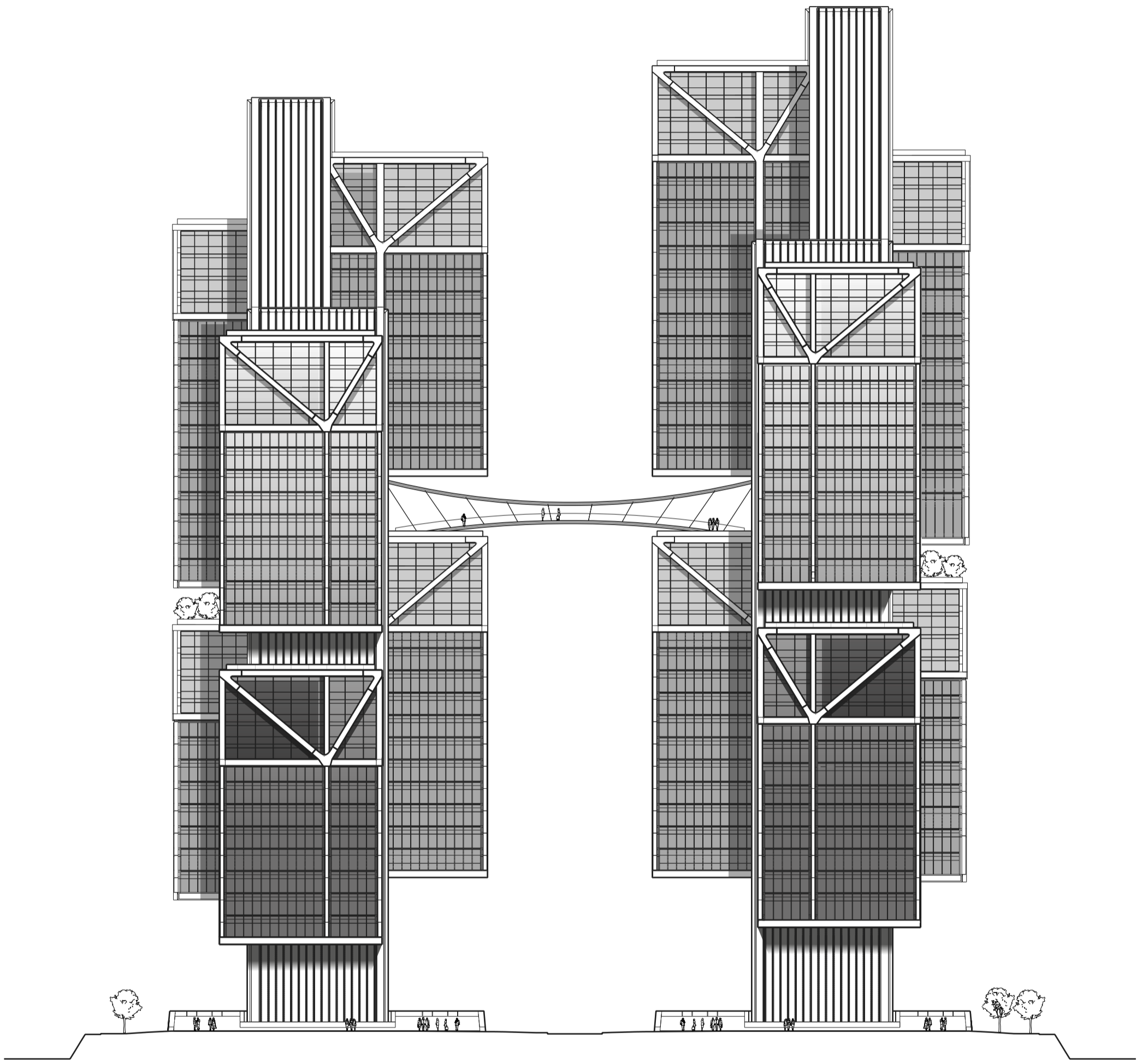
South Elevation
