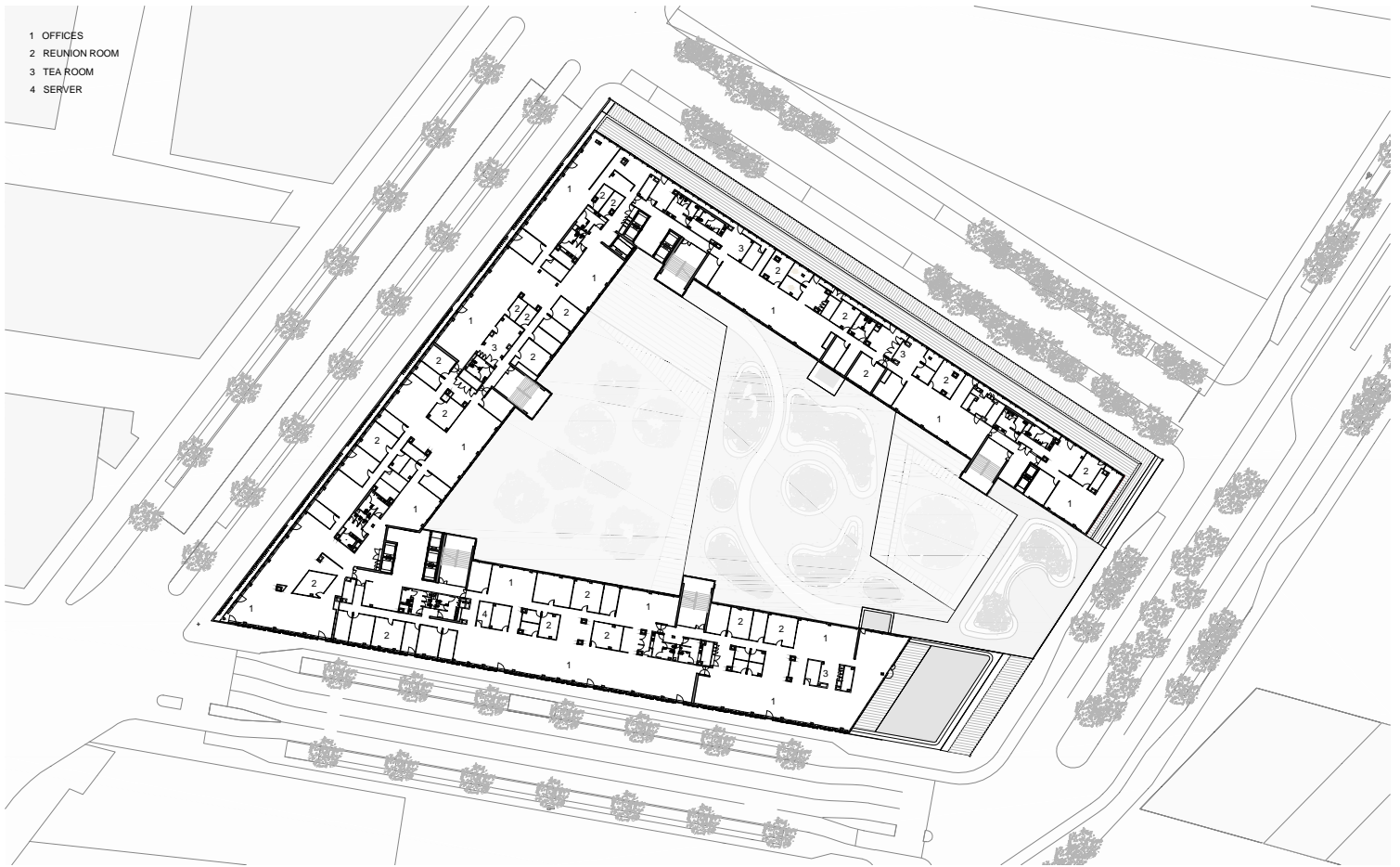
DFA | DIETMAR FEICHTINGER ARCHITECTES - AUBERVILLIERS - VEOLIA HEADQUARTERS - SIXTH LEVEL
