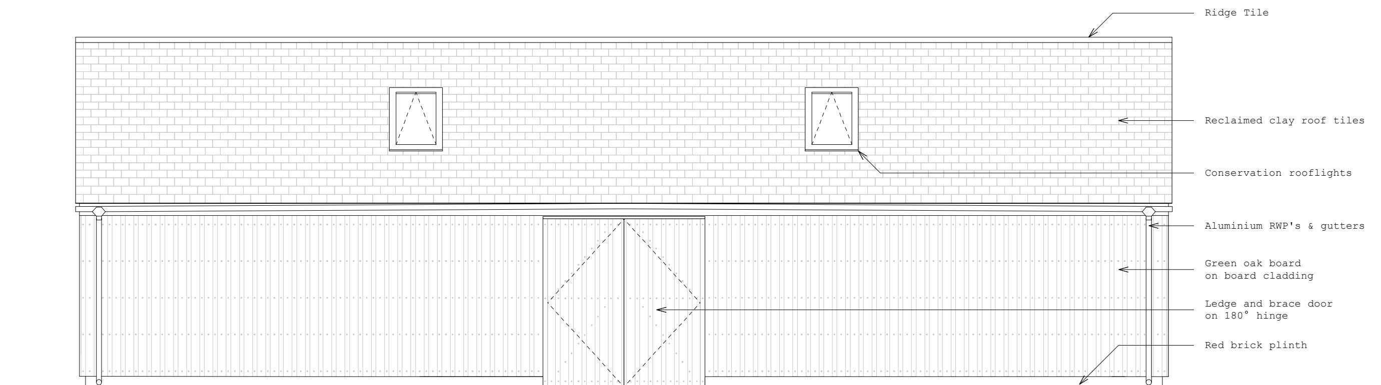
NORTH EAST ELEVATION 1:50 @ A3
