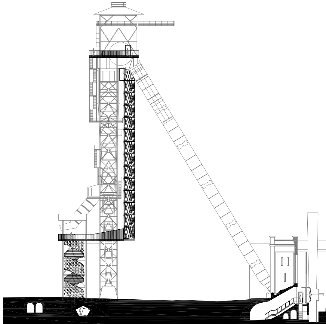
0 1 5 10 Section AA
