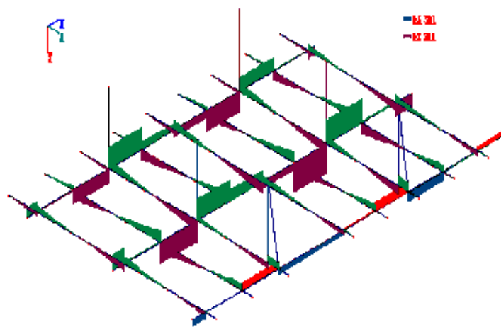
Shearing diagram
