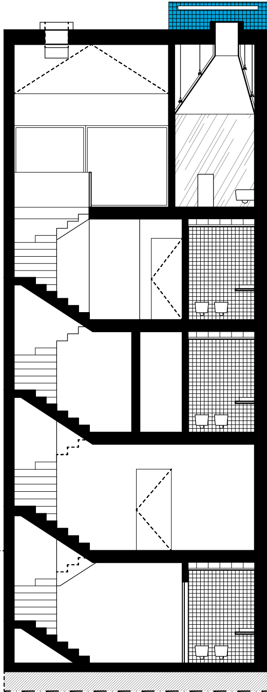
TRANSVERSAL SECTION
