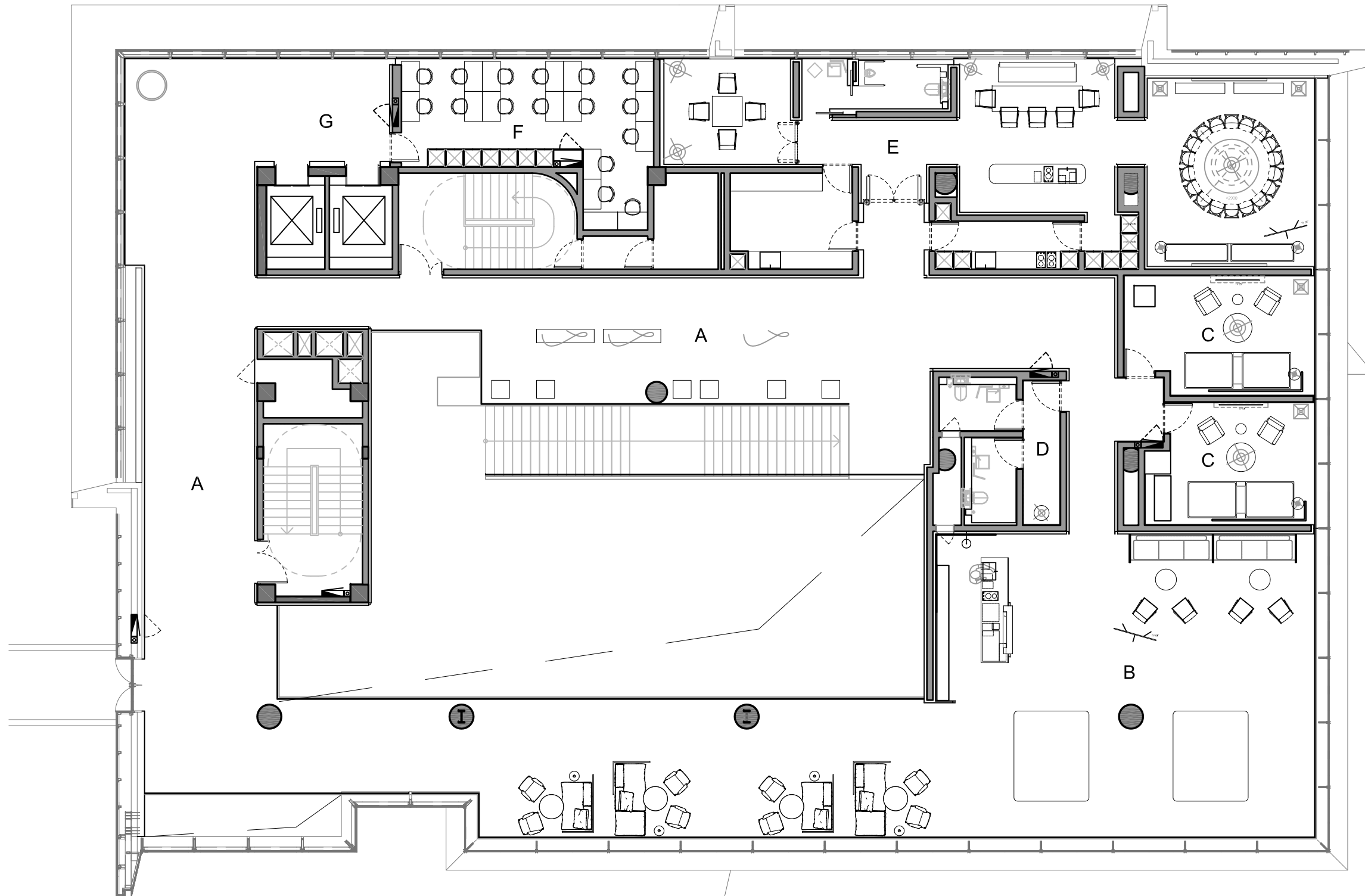
3F - Floor plan
