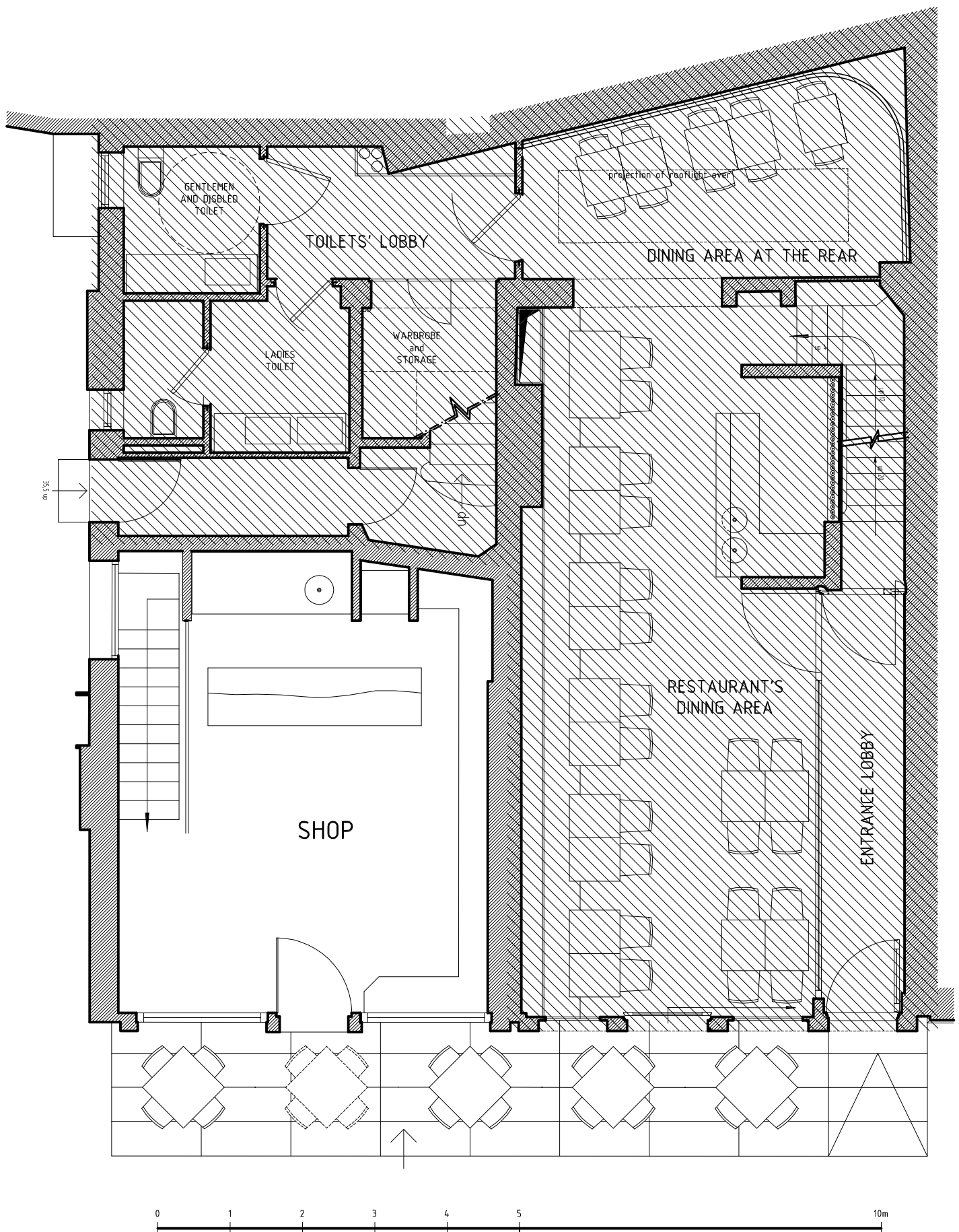
GROUND FLOOR PLAN OF Nr.10 and Nr.12 Lower Belgrave street
