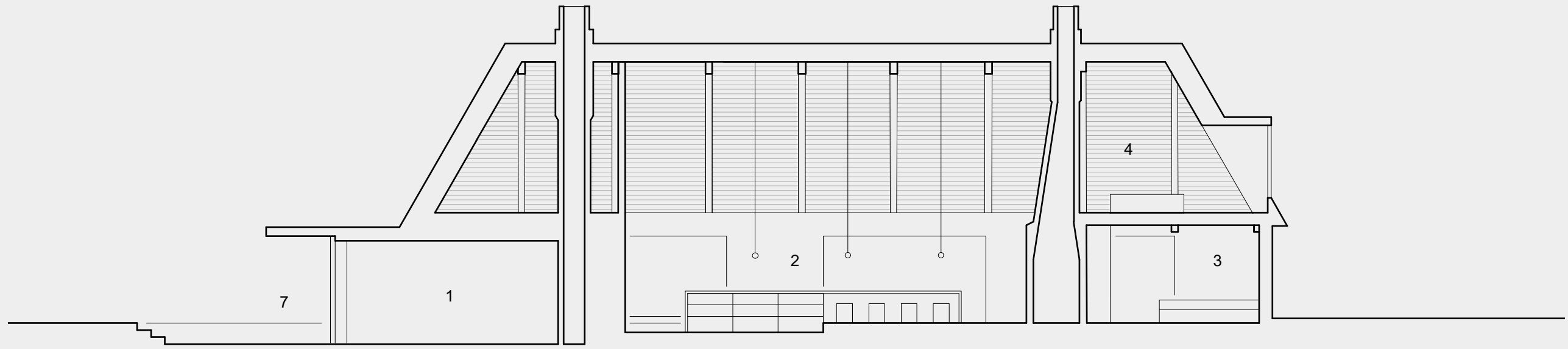
section aa
