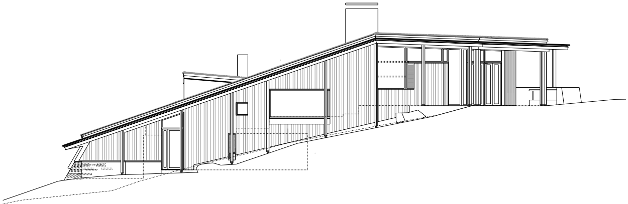
West elevation
