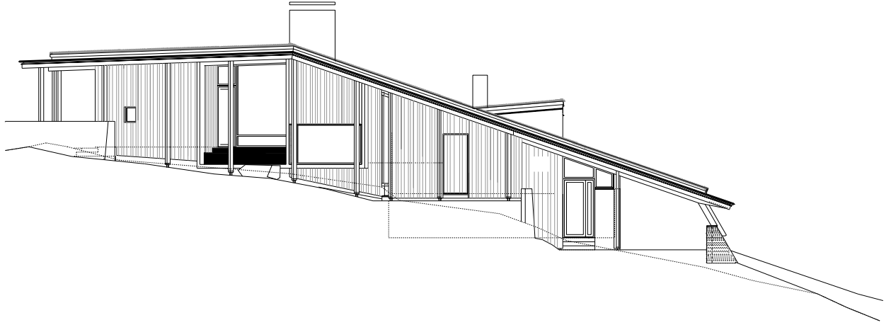
East elevation
