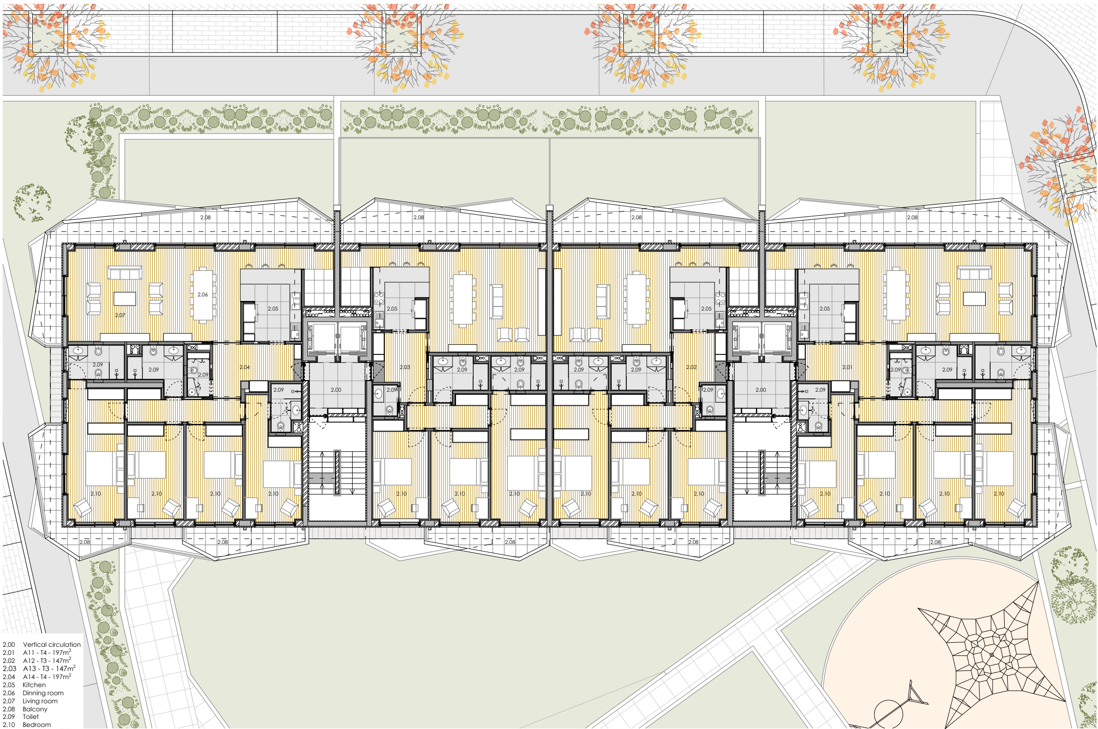
BUILDING A - TYPICAL FLOOR PLAN (2ND FLOOR)
