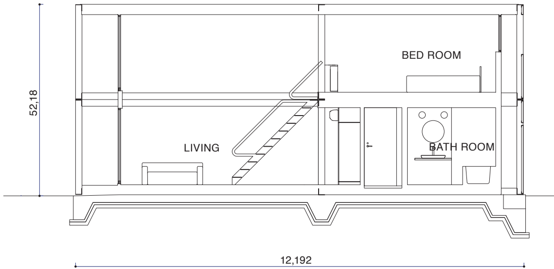
BAYSIDE MARINA HOTEL MAISONETTE TYPE UNIT SECTION 1/100
