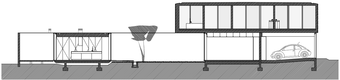
SECTION EE
