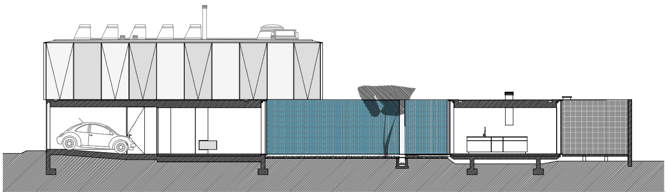
SECTION FF
