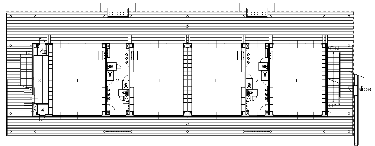
1st floor plan 1/300
