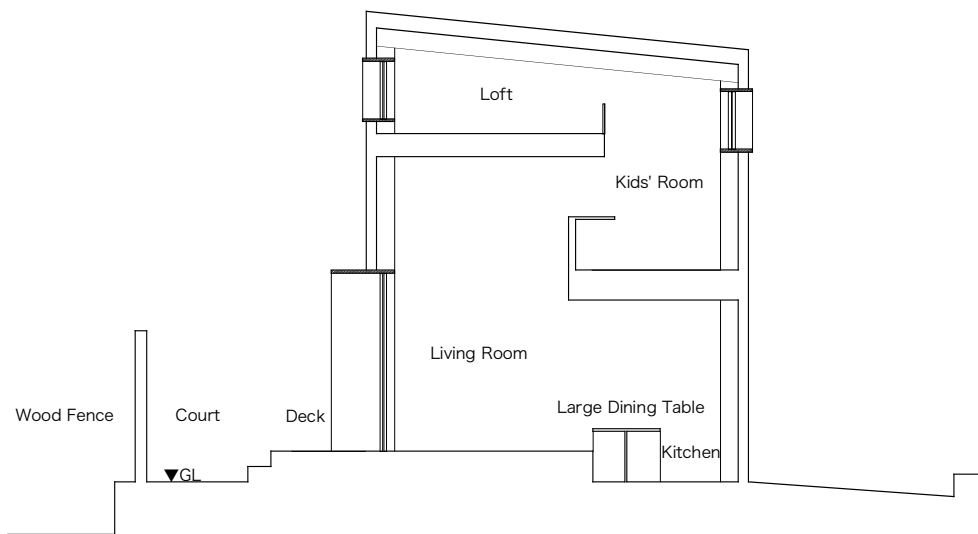
North-South Section 1
