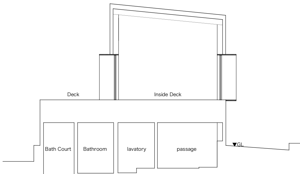
North-South Section 2
