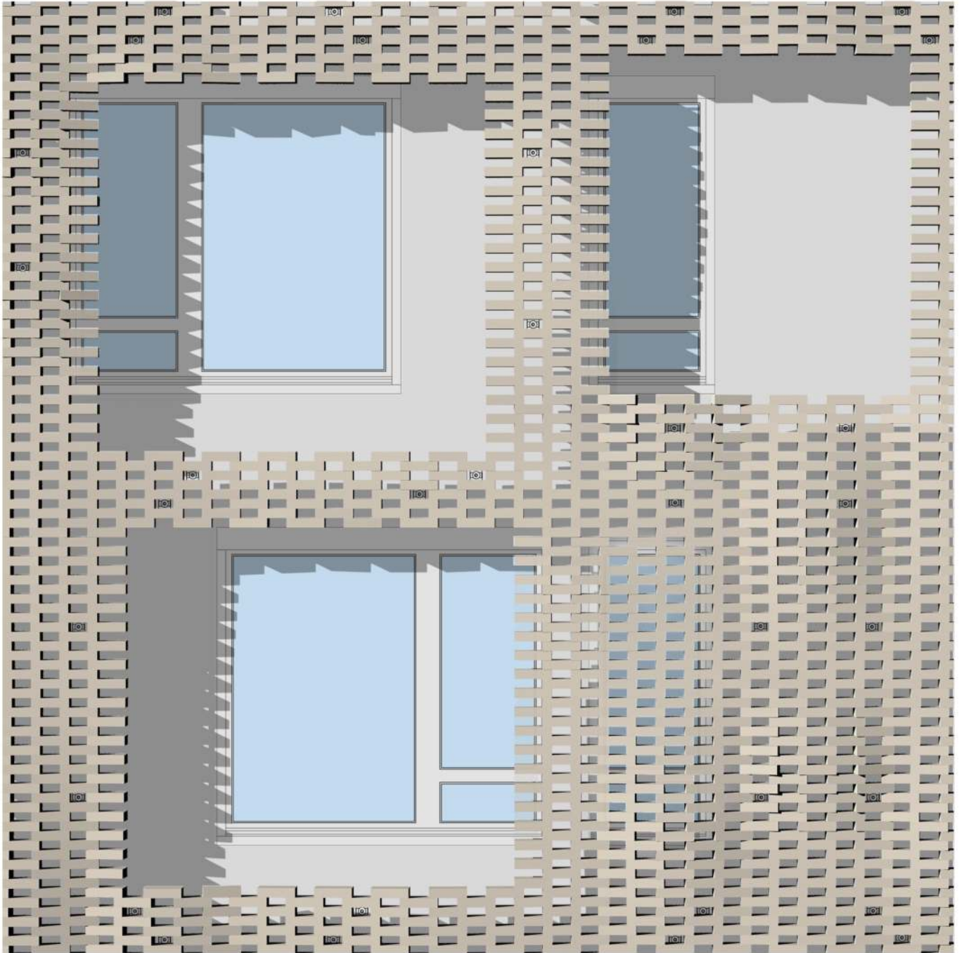
Facade concept 1:33
