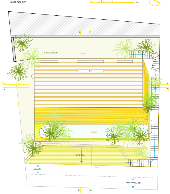
ROOF PLAN Level 720'-0"
