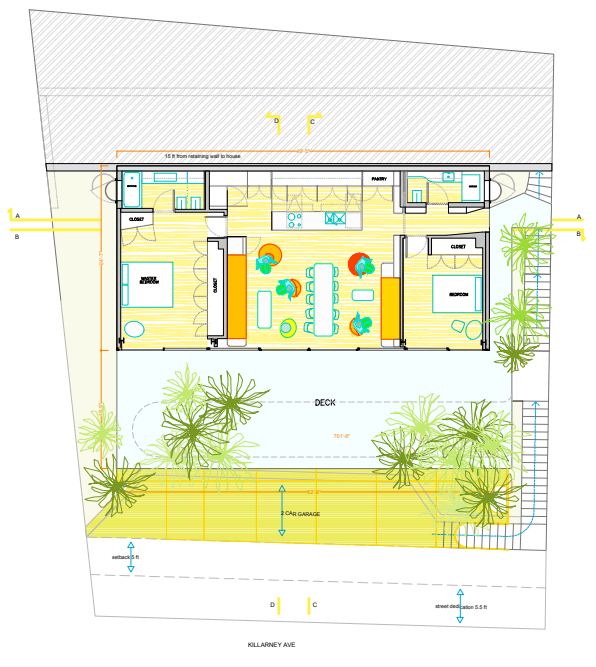
FIRST FLOOR PLAN Level 692'-2"
