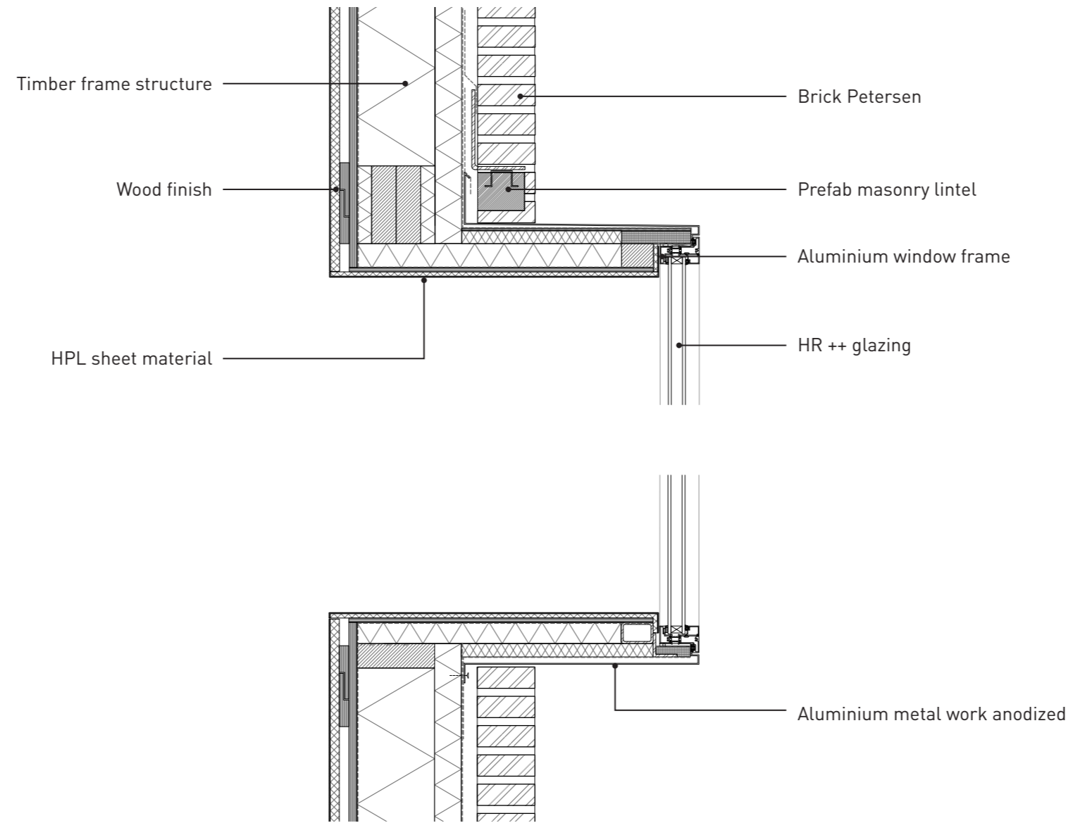
Detail window frame
