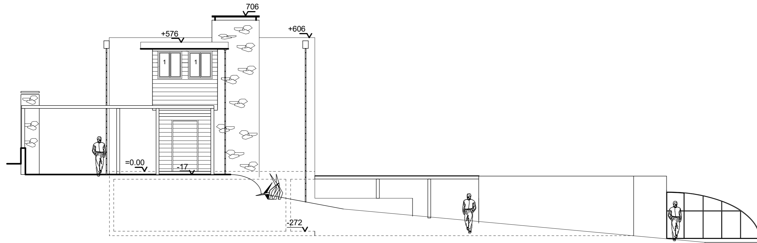
East elevation
