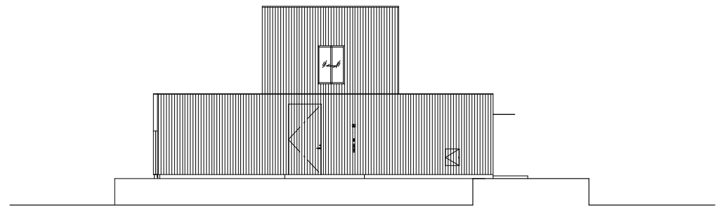
EAST ELEVATION
