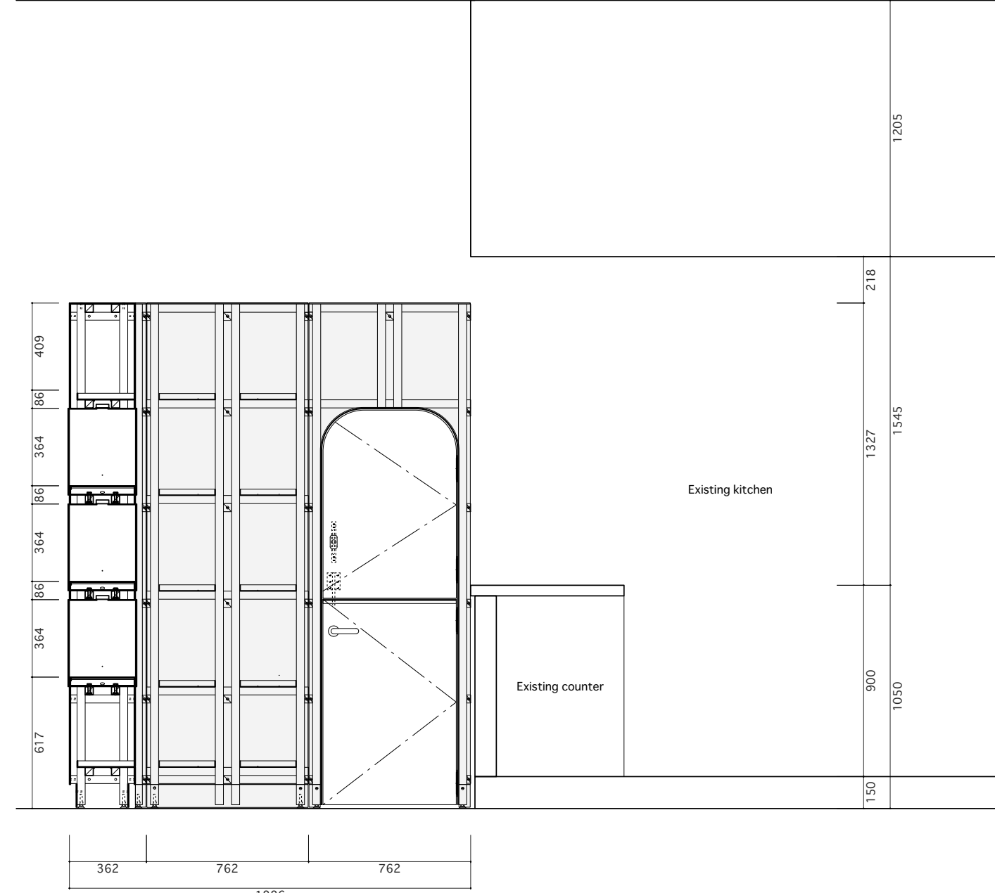
Section B-B'
