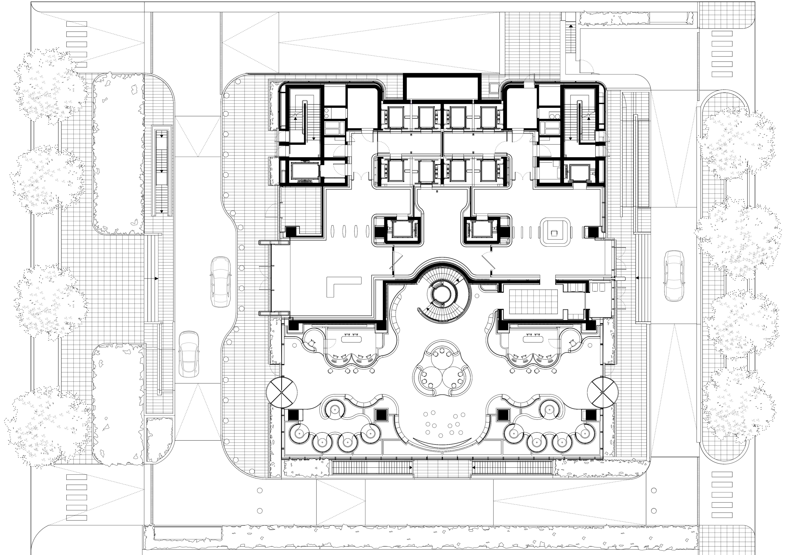
Techcombank HCMC - Floorplan Level 01
