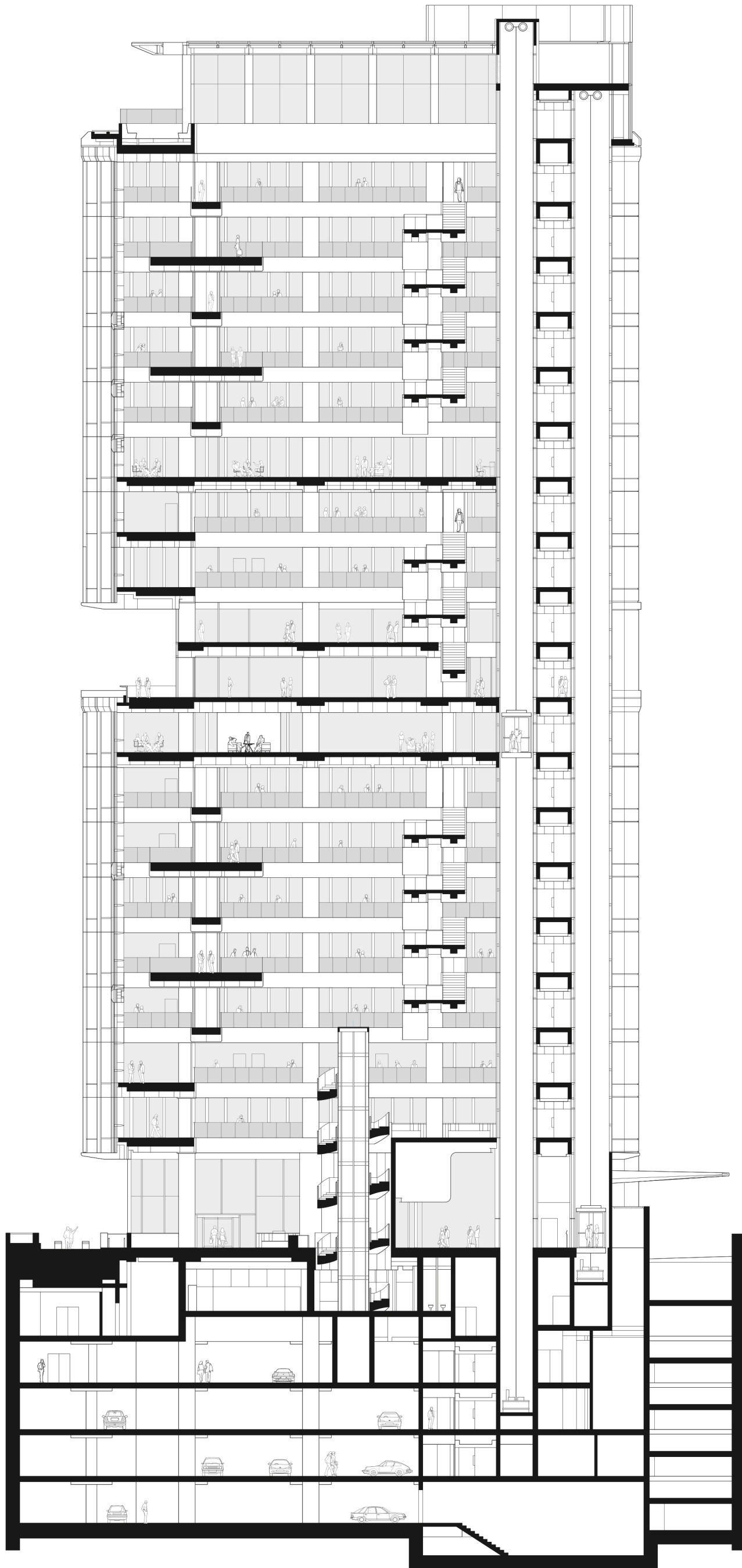
Techcombank HCMC - Longitudinal Cross Section
