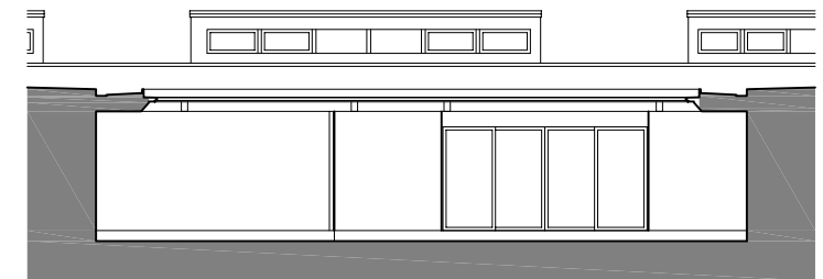
west elevation - Courtyard
