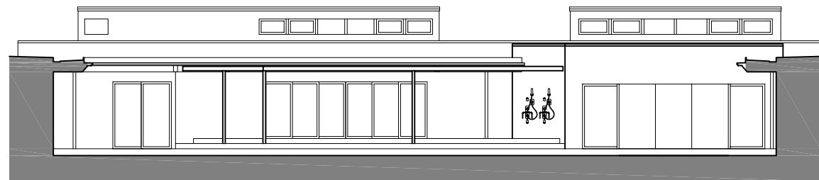
east elevational - Courtyard
