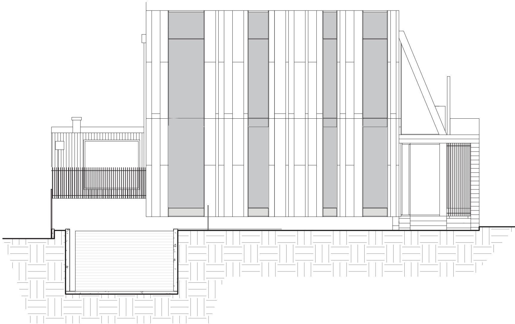
SOUTH ELEVATION
