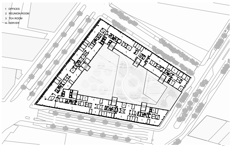
DFA | DIETMAR FEICHTINGER ARCHITECTES - AUBERVILLIERS - VEOLIA HEADQUARTERS - THIRD LEVEL
