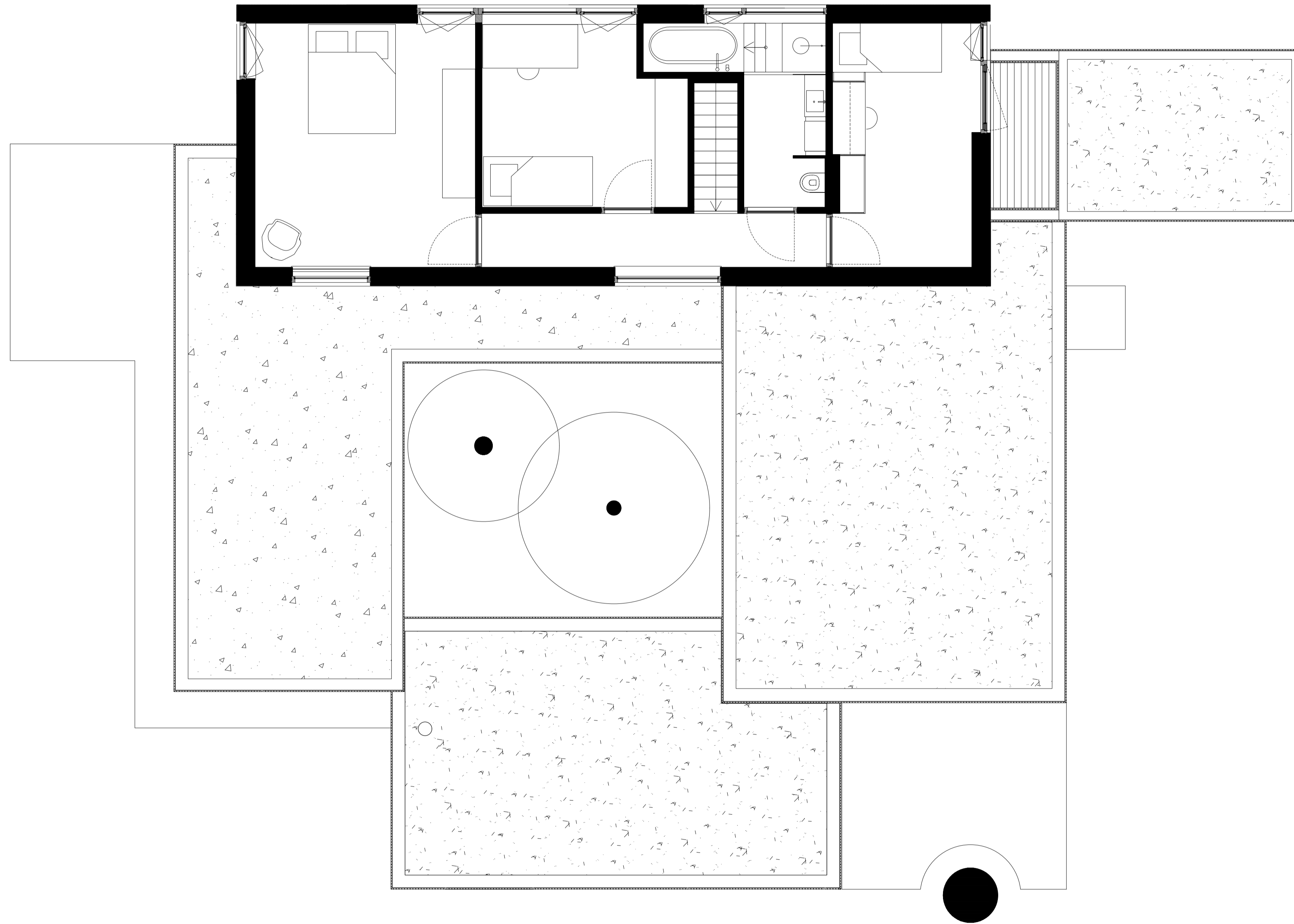
VERDIEPING / FIRST FLOOR
