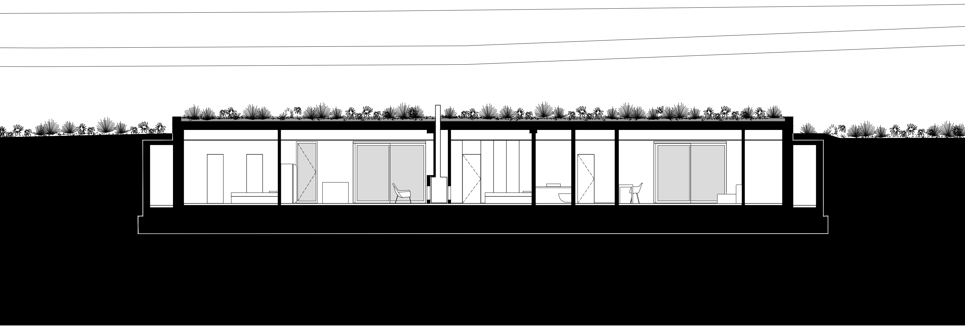
0 1m 2 3 SECTION B
