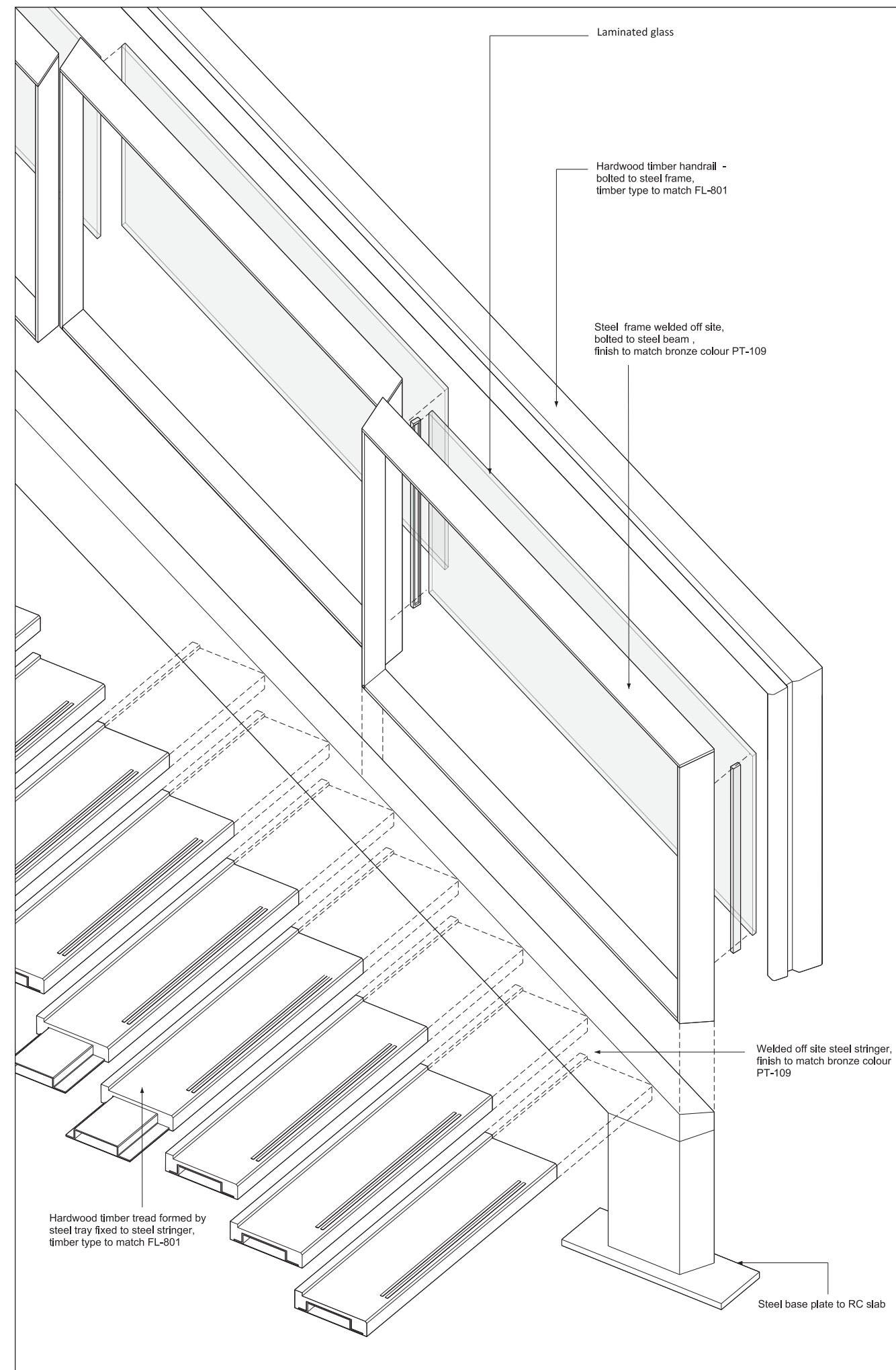
02 NTS Exploded Stair Axo View
