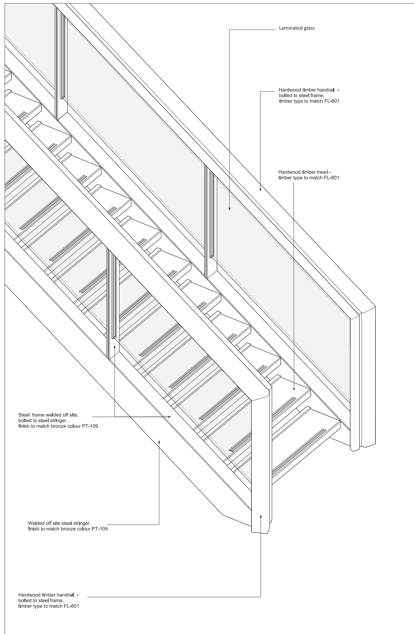
01 NTS Stair Axo View
