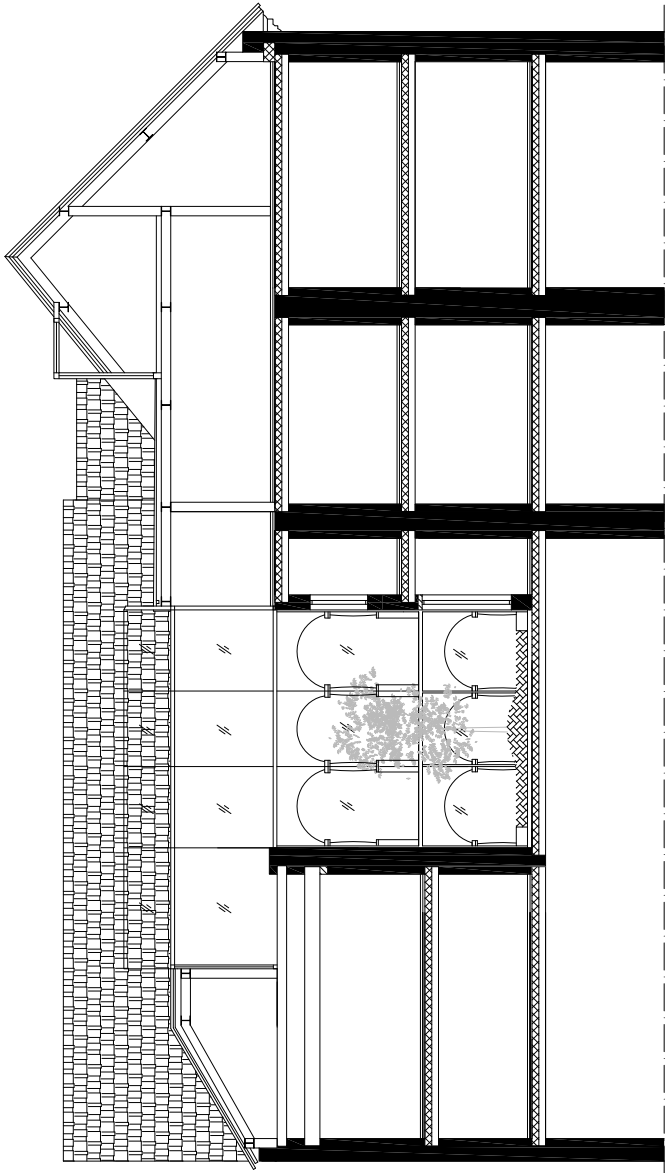
SECTION B-B
