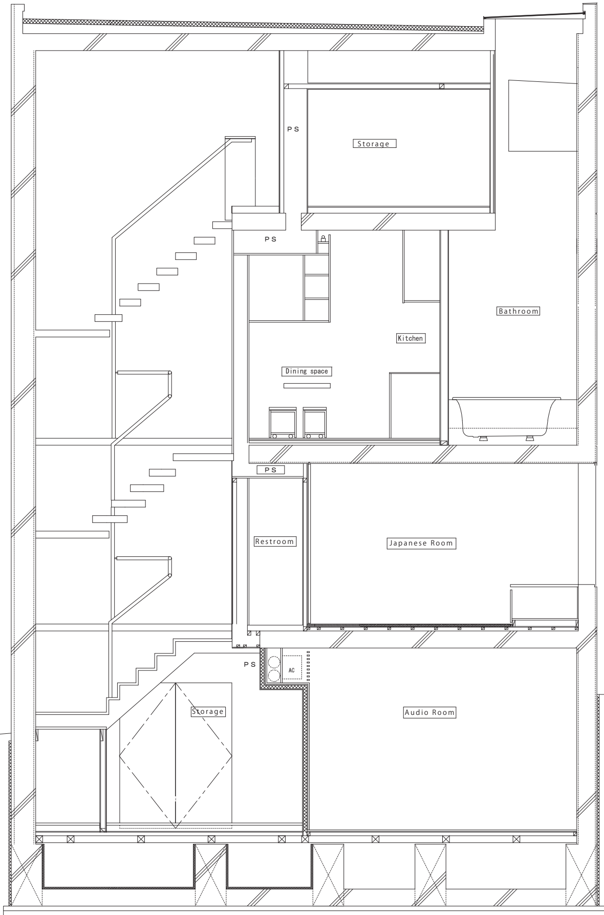
Section S=1/50
