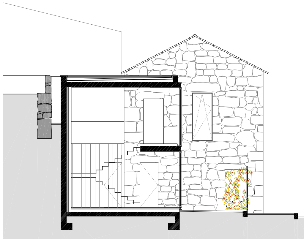
CROSS SECTION
