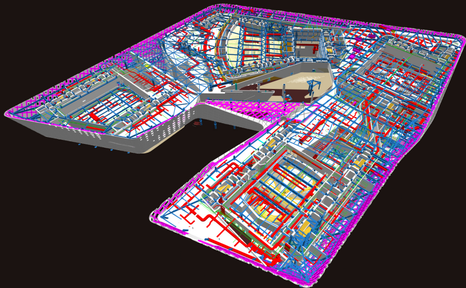
Nanjing International Youth Cultural Centre BIM MODEL - Section
