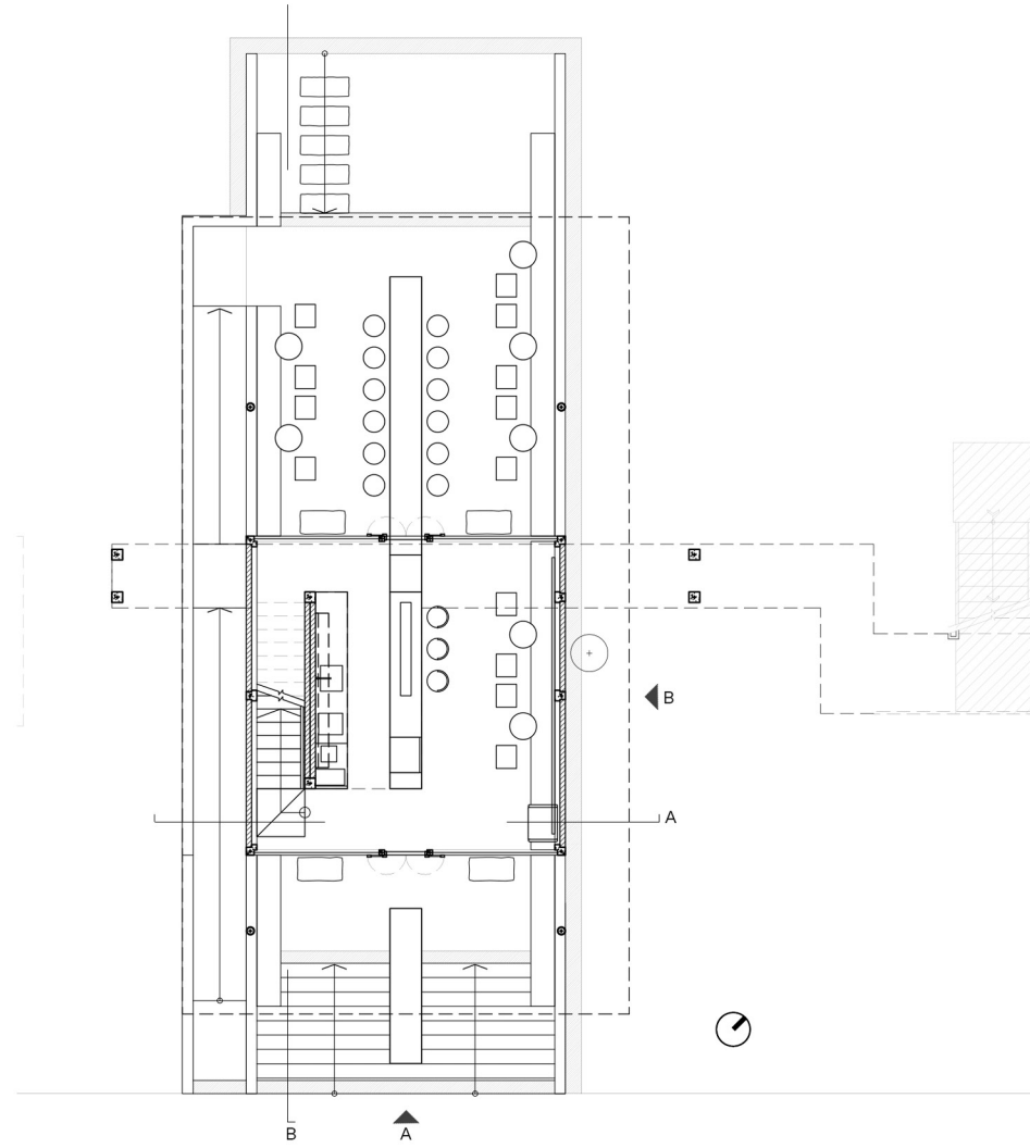
1F Plan
