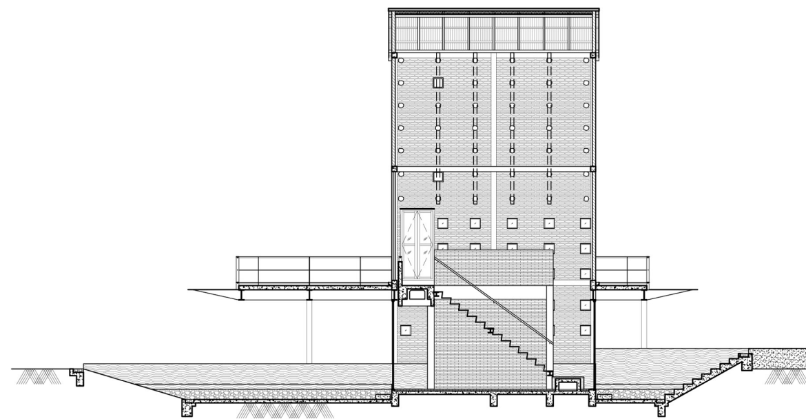
Section
