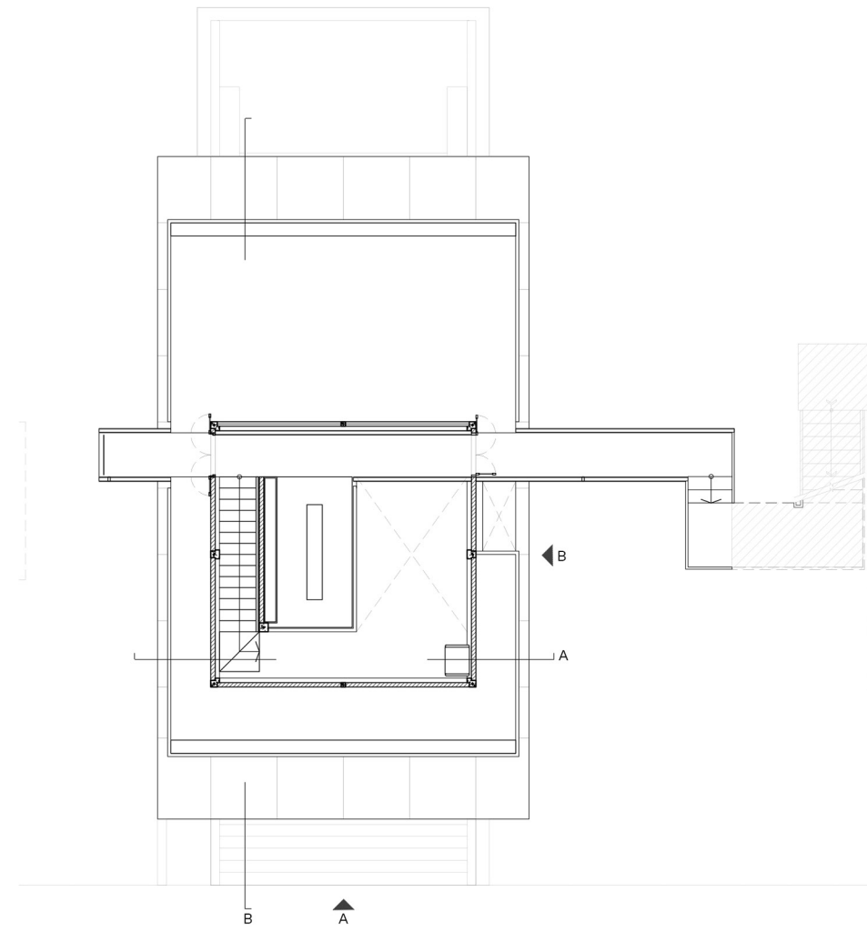
2F Plan
