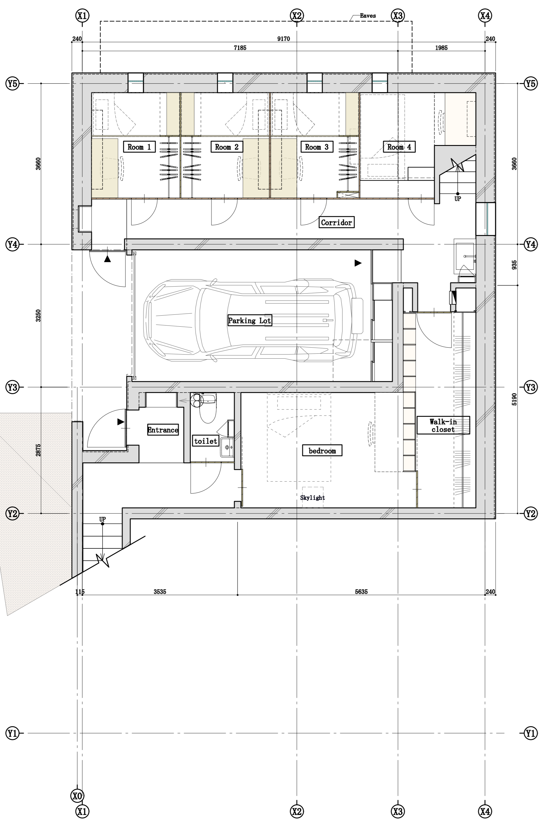
Basement 1st floor plan
