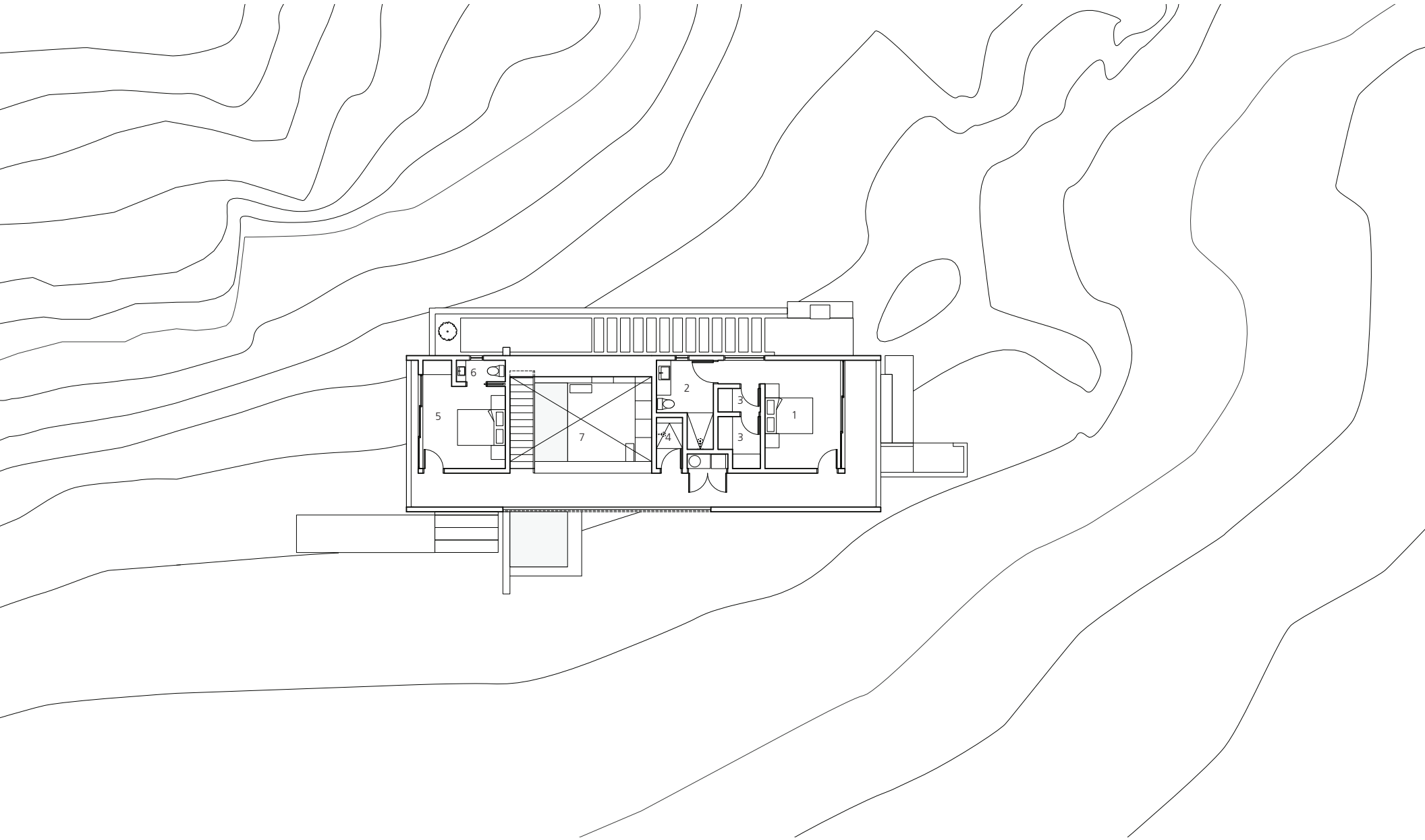
Upper Floor Plan 1-master bedroom 2-master ensuite 3-closet 4-shower 5-bedroom 6-ensuite 7-open to below
