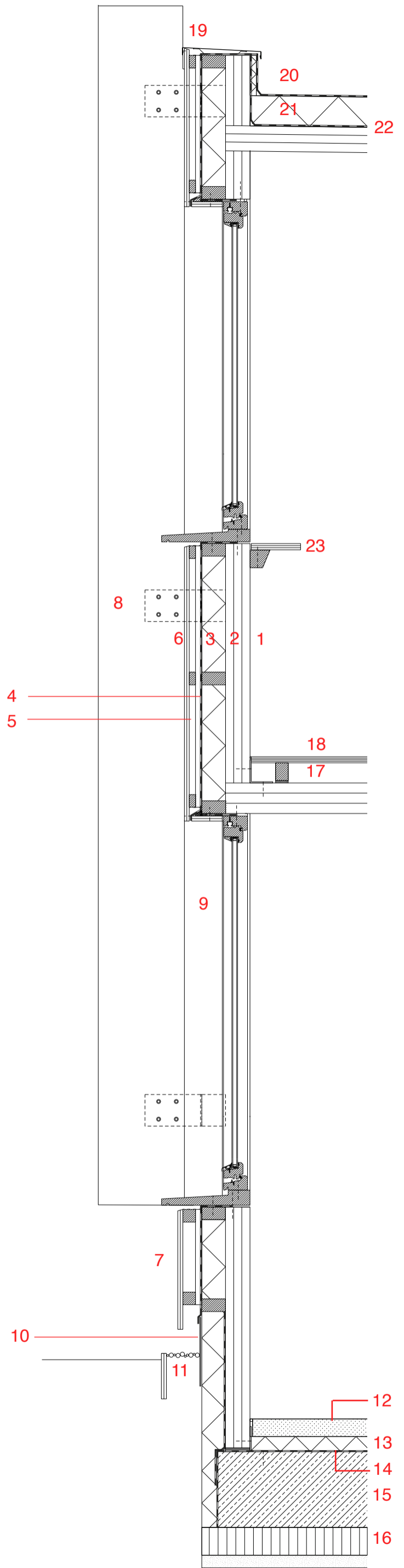
FACADE DETAIL
